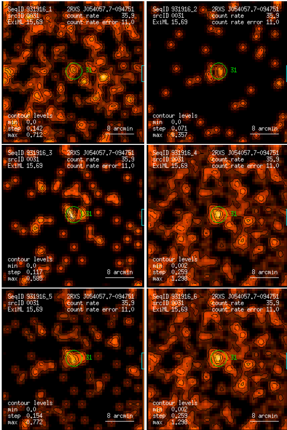
Figure 31: RASS 931916: detection 0031: band rate images, Gaussian filter: (1) PSPC channels 11 – 41, (2) 52 – 90, (3) 91 – 201, (4) 11 – 235, (5) 52 – 201, (6) 11 – 201. Broad band rates in counts/ks. Band rate contour levels in counts/ks/arcmin 2 .
