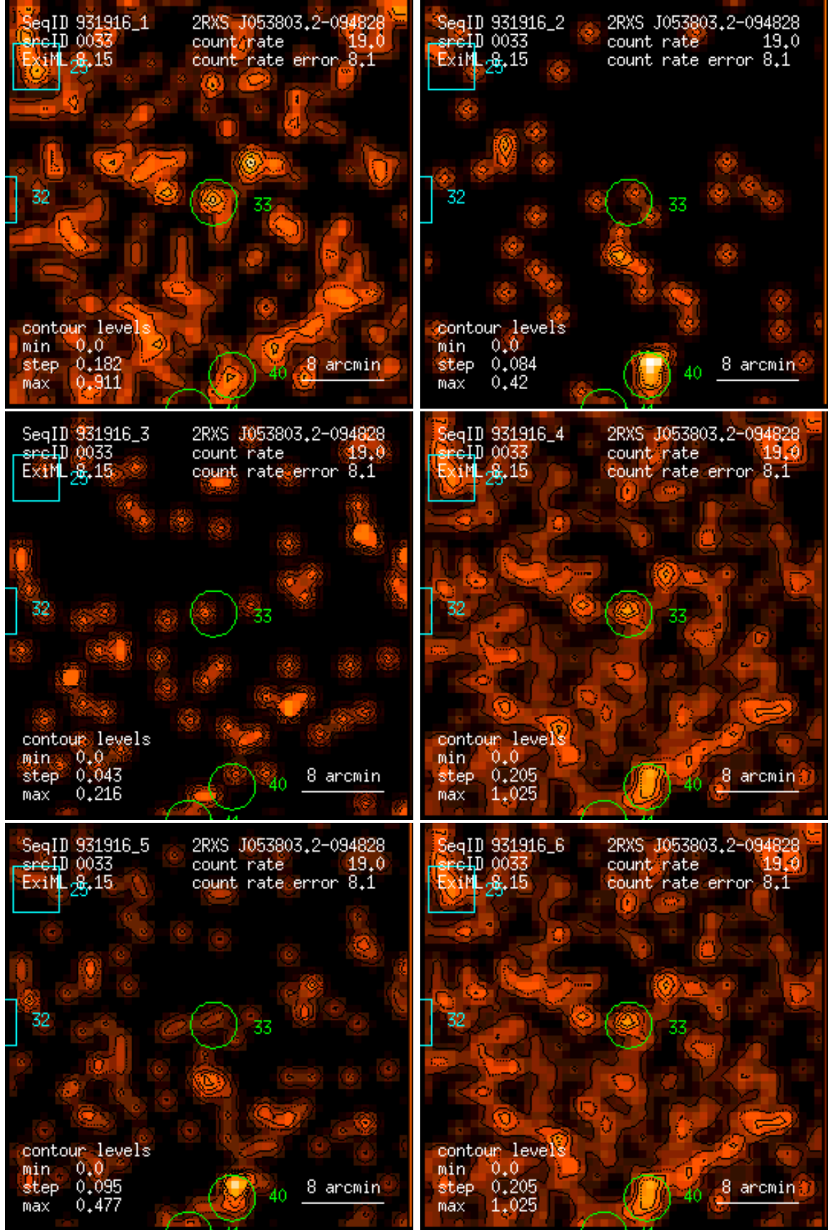
Figure 33: RASS 931916: detection 0033: band rate images, Gaussian filter: (1) PSPC channels 11 – 41, (2) 52 – 90, (3) 91 – 201, (4) 11 – 235, (5) 52 – 201, (6) 11 – 201. Broad band rates in counts/ks. Band rate contour levels in counts/ks/arcmin 2 .
