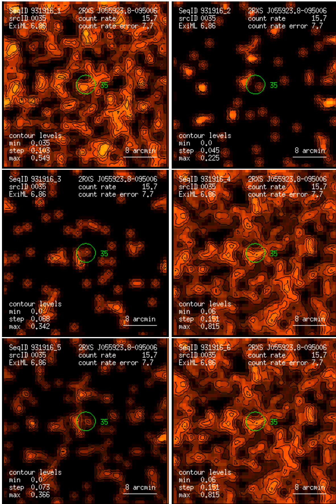
Figure 35: RASS 931916: detection 0035: band rate images, Gaussian filter: (1) PSPC channels 11 – 41, (2) 52 – 90, (3) 91 – 201, (4) 11 – 235, (5) 52 – 201, (6) 11 – 201. Broad band rates in counts/ks. Band rate contour levels in counts/ks/arcmin 2 .
