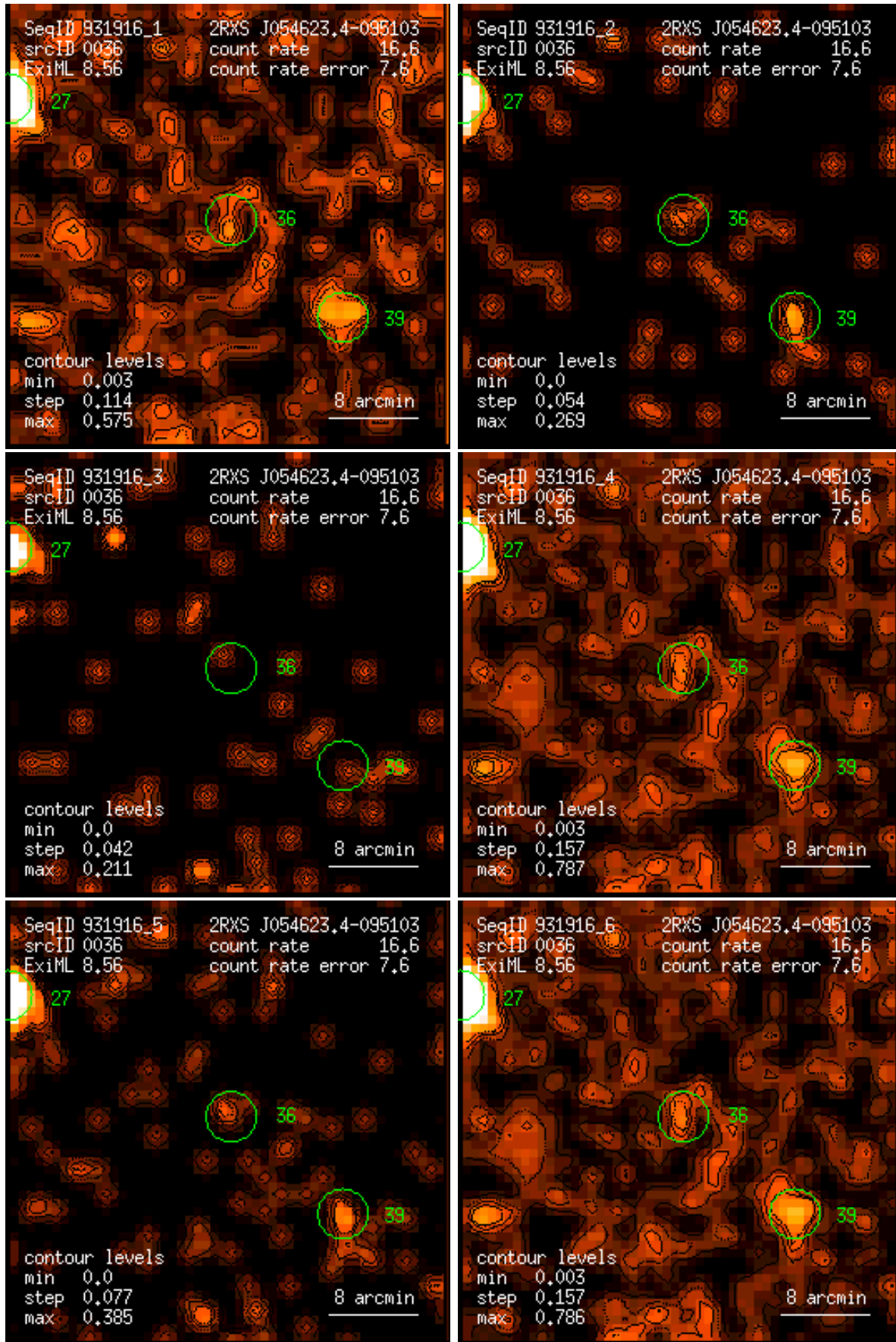
Figure 36: RASS 931916: detection 0036: band rate images, Gaussian filter: (1) PSPC channels 11 – 41, (2) 52 – 90, (3) 91 – 201, (4) 11 – 235, (5) 52 – 201, (6) 11 – 201. Broad band rates in counts/ks. Band rate contour levels in counts/ks/arcmin 2 .
