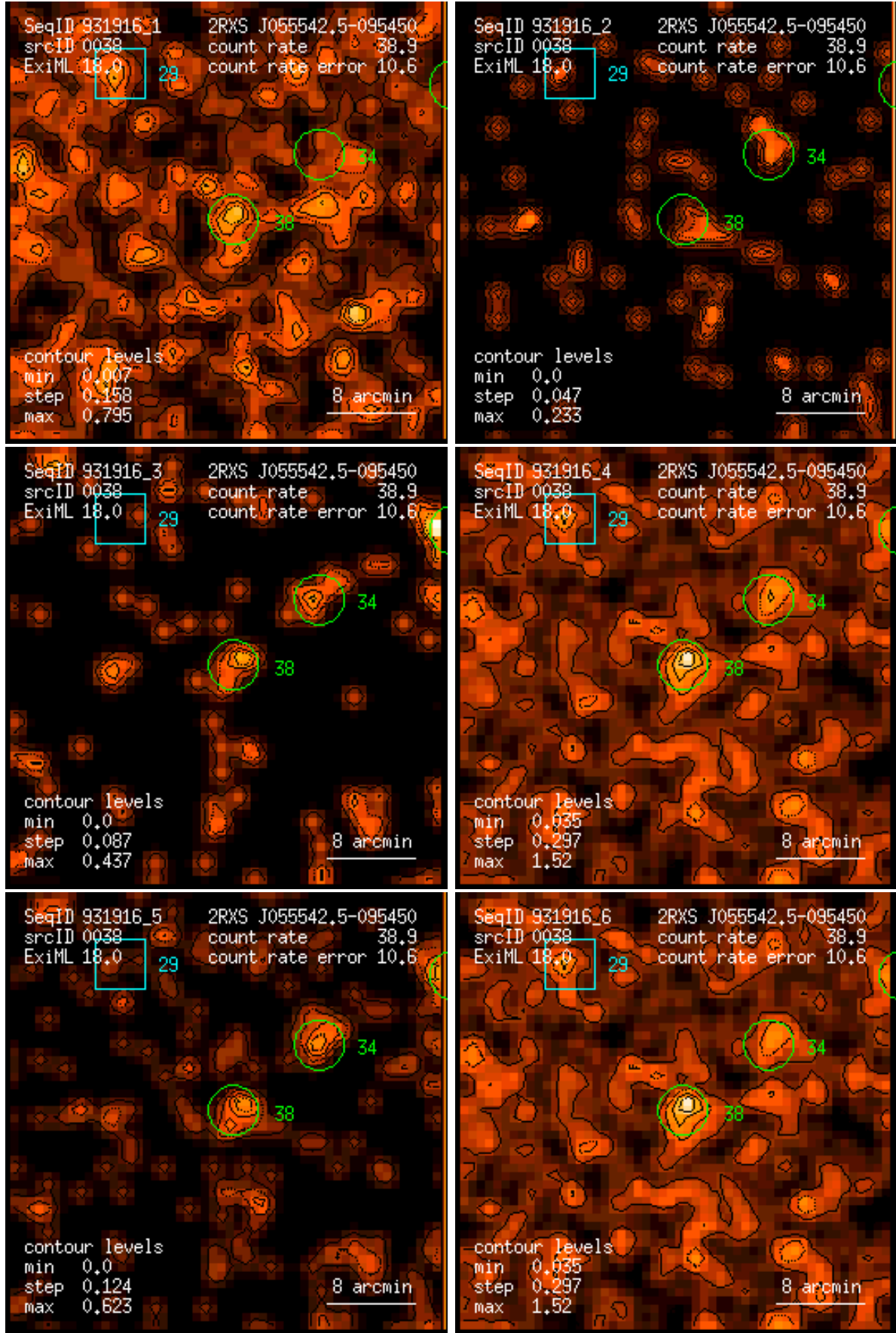
Figure 38: RASS 931916: detection 0038: band rate images, Gaussian filter: (1) PSPC channels 11 – 41, (2) 52 – 90, (3) 91 – 201, (4) 11 – 235, (5) 52 – 201, (6) 11 – 201. Broad band rates in counts/ks. Band rate contour levels in counts/ks/arcmin 2 .
