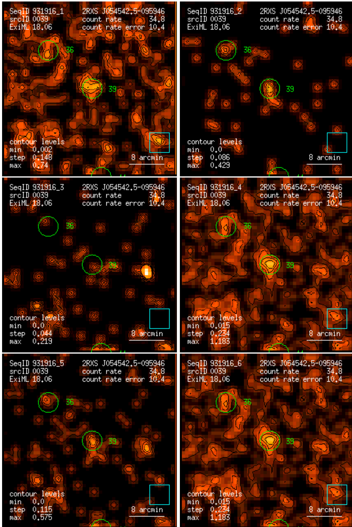
Figure 39: RASS 931916: detection 0039: band rate images, Gaussian filter: (1) PSPC channels 11 – 41, (2) 52 – 90, (3) 91 – 201, (4) 11 – 235, (5) 52 – 201, (6) 11 – 201. Broad band rates in counts/ks. Band rate contour levels in counts/ks/arcmin 2 .
