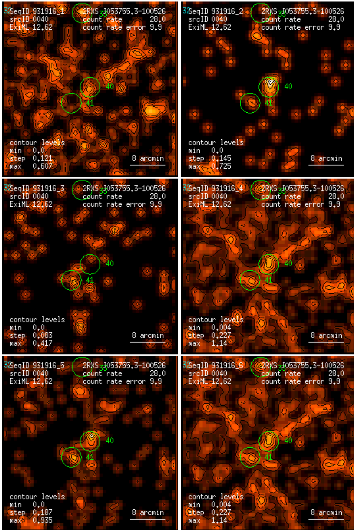
Figure 40: RASS 931916: detection 0040: band rate images, Gaussian filter: (1) PSPC channels 11 – 41, (2) 52 – 90, (3) 91 – 201, (4) 11 – 235, (5) 52 – 201, (6) 11 – 201. Broad band rates in counts/ks. Band rate contour levels in counts/ks/arcmin 2 .
