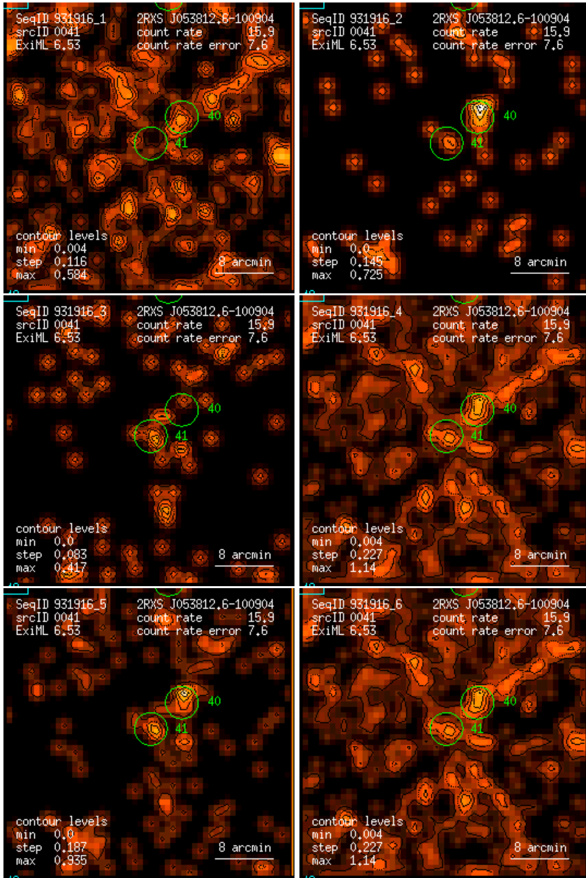
Figure 41: RASS 931916: detection 0041: band rate images, Gaussian filter: (1) PSPC channels 11 – 41, (2) 52 – 90, (3) 91 – 201, (4) 11 – 235, (5) 52 – 201, (6) 11 – 201. Broad band rates in counts/ks. Band rate contour levels in counts/ks/arcmin 2 .
