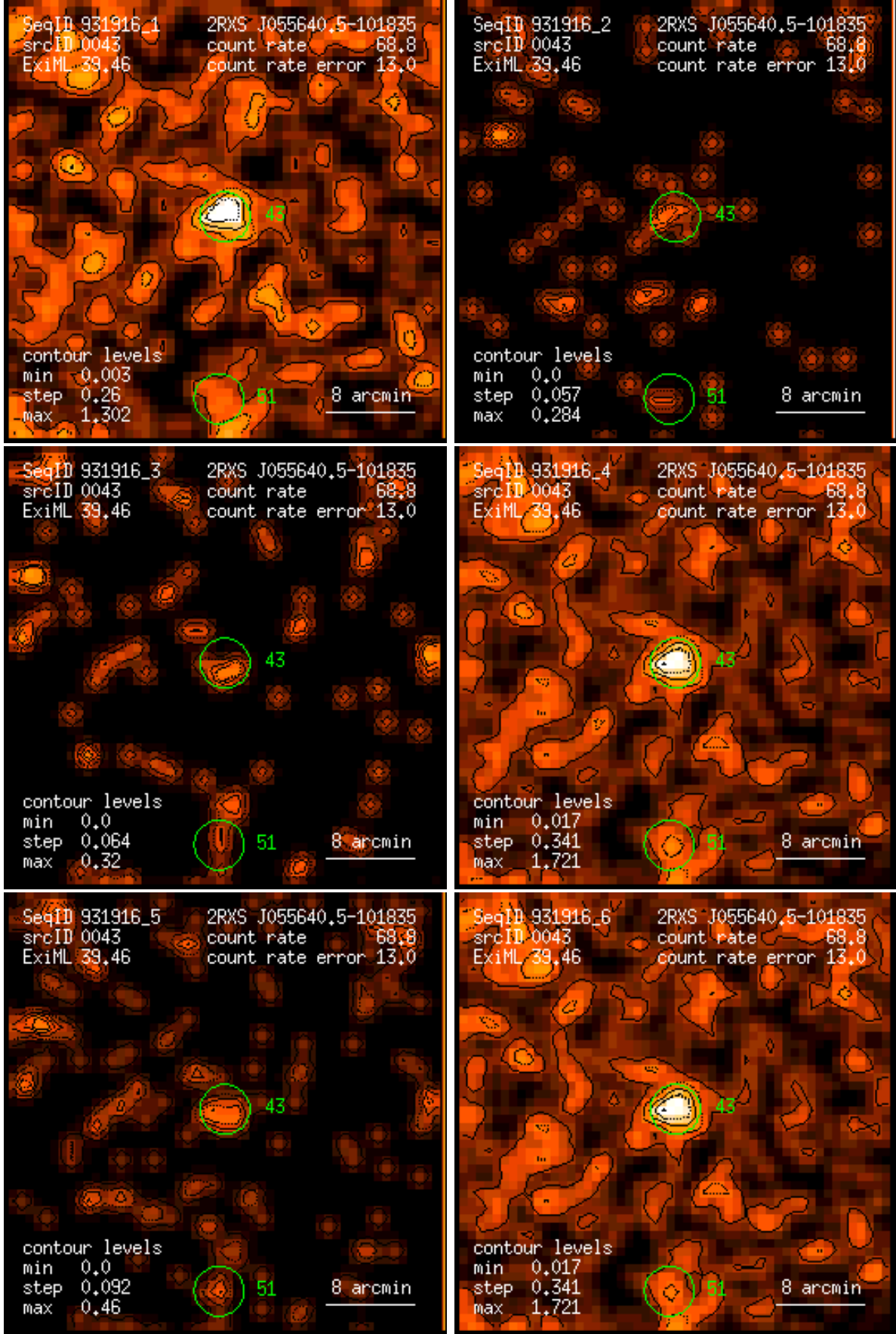
Figure 43: RASS 931916: detection 0043: band rate images, Gaussian filter: (1) PSPC channels 11 – 41, (2) 52 – 90, (3) 91 – 201, (4) 11 – 235, (5) 52 – 201, (6) 11 – 201. Broad band rates in counts/ks. Band rate contour levels in counts/ks/arcmin 2 .
