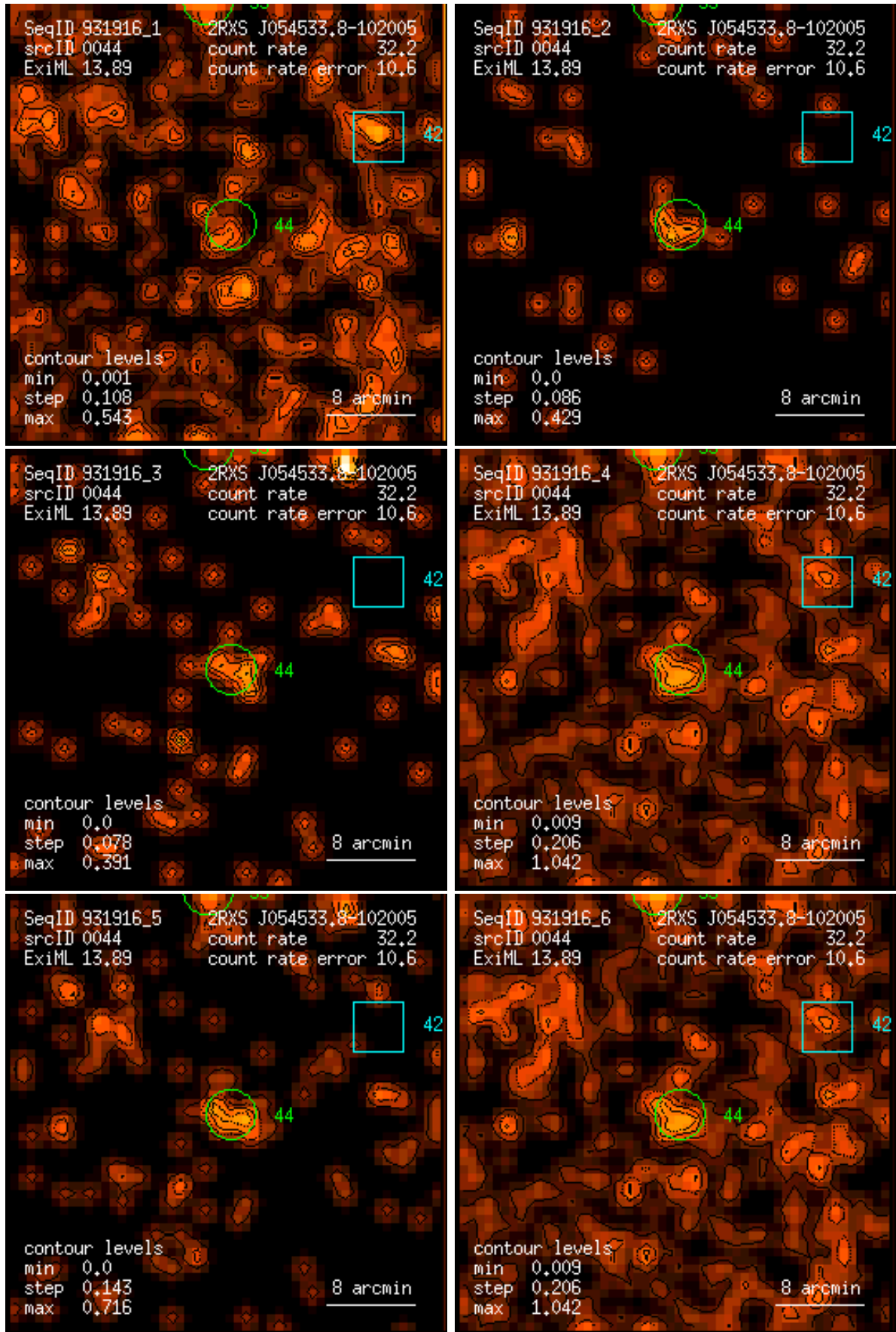
Figure 44: RASS 931916: detection 0044: band rate images, Gaussian filter: (1) PSPC channels 11 – 41, (2) 52 – 90, (3) 91 – 201, (4) 11 – 235, (5) 52 – 201, (6) 11 – 201. Broad band rates in counts/ks. Band rate contour levels in counts/ks/arcmin 2 .
