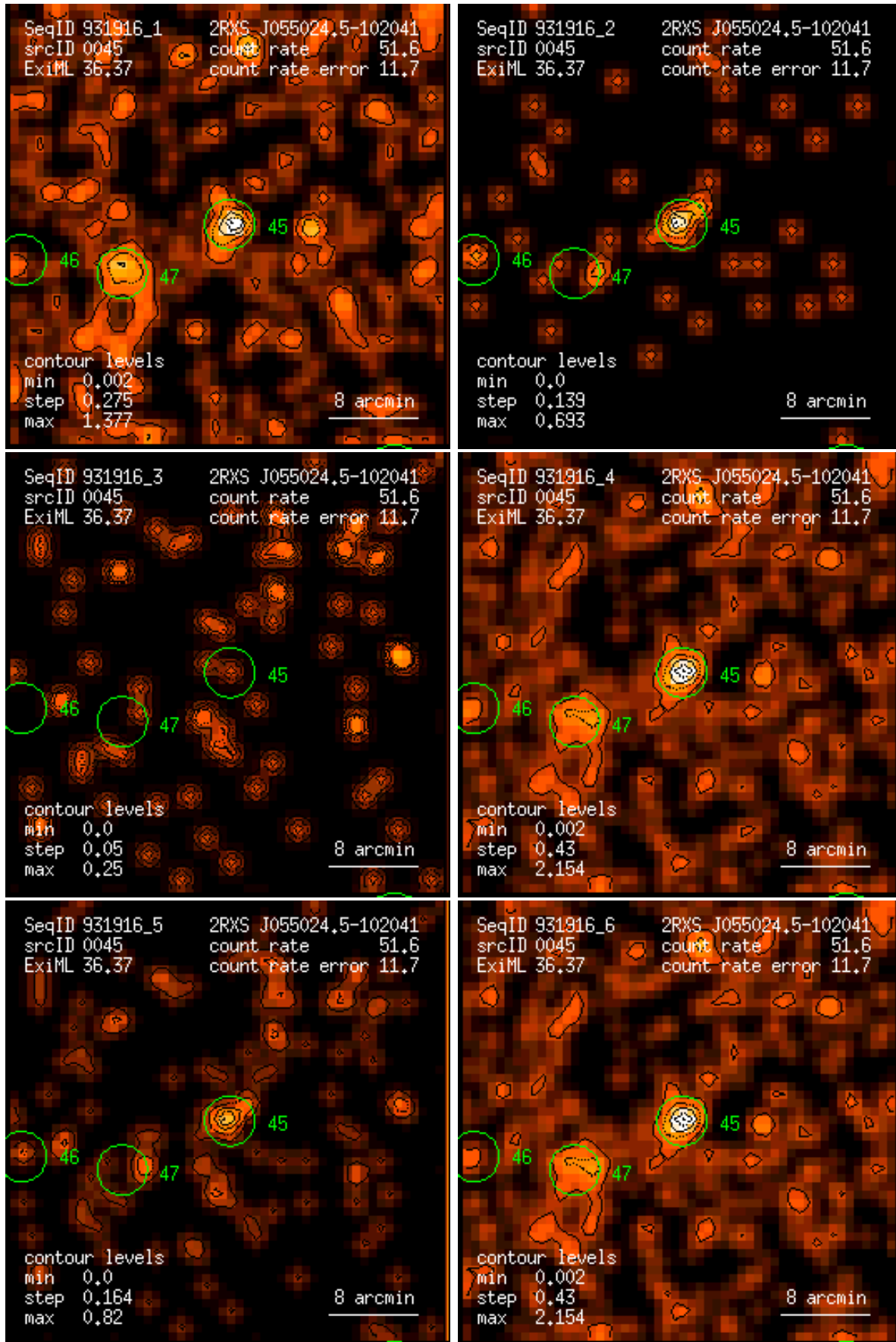
Figure 45: RASS 931916: detection 0045: band rate images, Gaussian filter: (1) PSPC channels 11 – 41, (2) 52 – 90, (3) 91 – 201, (4) 11 – 235, (5) 52 – 201, (6) 11 – 201. Broad band rates in counts/ks. Band rate contour levels in counts/ks/arcmin 2 .
