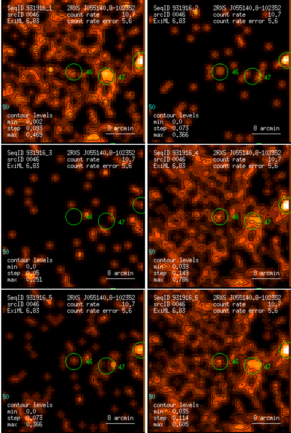
Figure 46: RASS 931916: detection 0046: band rate images, Gaussian filter: (1) PSPC channels 11 – 41, (2) 52 – 90, (3) 91 – 201, (4) 11 – 235, (5) 52 – 201, (6) 11 – 201. Broad band rates in counts/ks. Band rate contour levels in counts/ks/arcmin 2 .
