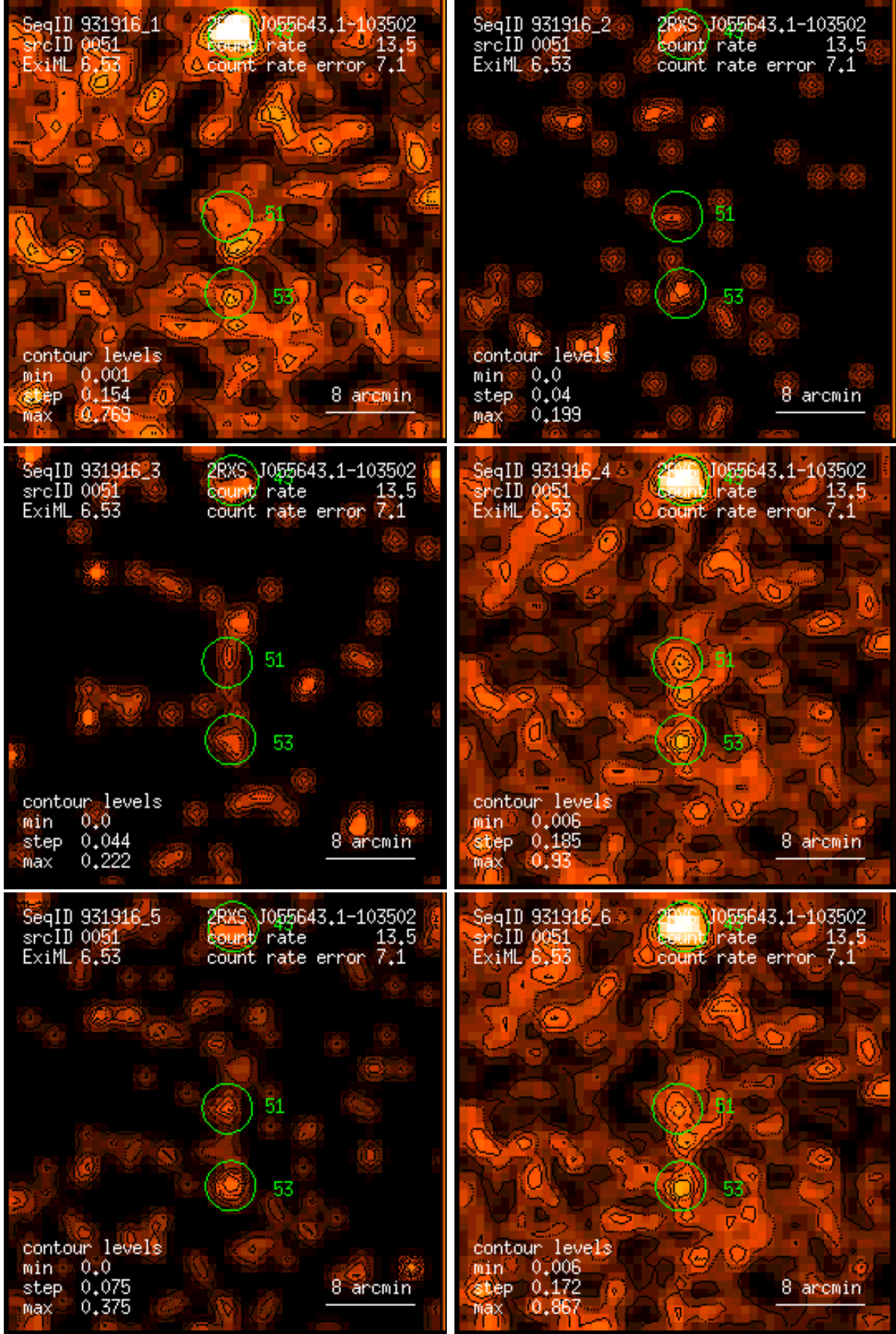
Figure 51: RASS 931916: detection 0051: band rate images, Gaussian filter: (1) PSPC channels 11 – 41, (2) 52 – 90, (3) 91 – 201, (4) 11 – 235, (5) 52 – 201, (6) 11 – 201. Broad band rates in counts/ks. Band rate contour levels in counts/ks/arcmin 2 .
