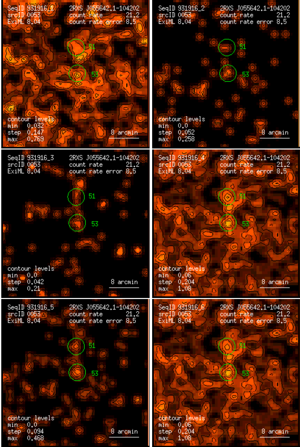
Figure 53: RASS 931916: detection 0053: band rate images, Gaussian filter: (1) PSPC channels 11 – 41, (2) 52 – 90, (3) 91 – 201, (4) 11 – 235, (5) 52 – 201, (6) 11 – 201. Broad band rates in counts/ks. Band rate contour levels in counts/ks/arcmin 2 .
