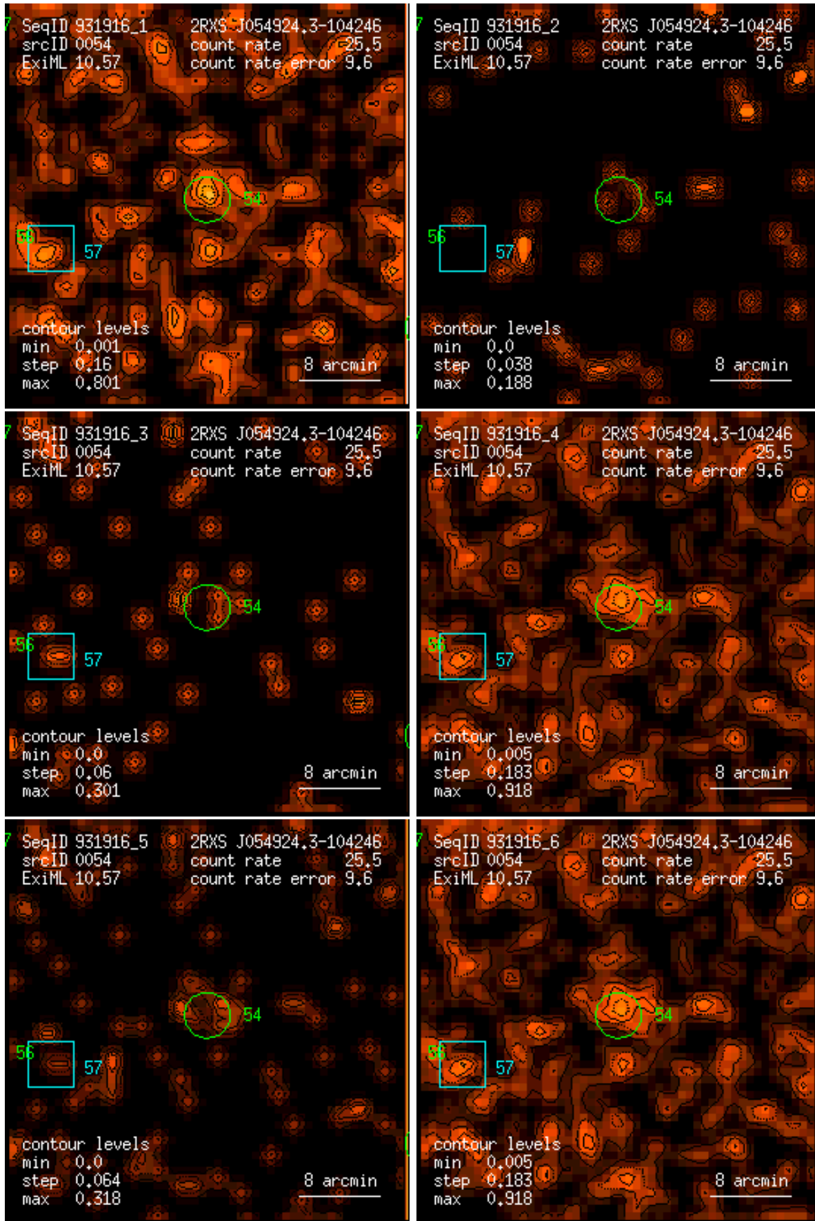
Figure 54: RASS 931916: detection 0054: band rate images, Gaussian filter: (1) PSPC channels 11 – 41, (2) 52 – 90, (3) 91 – 201, (4) 11 – 235, (5) 52 – 201, (6) 11 – 201. Broad band rates in counts/ks. Band rate contour levels in counts/ks/arcmin 2 .
