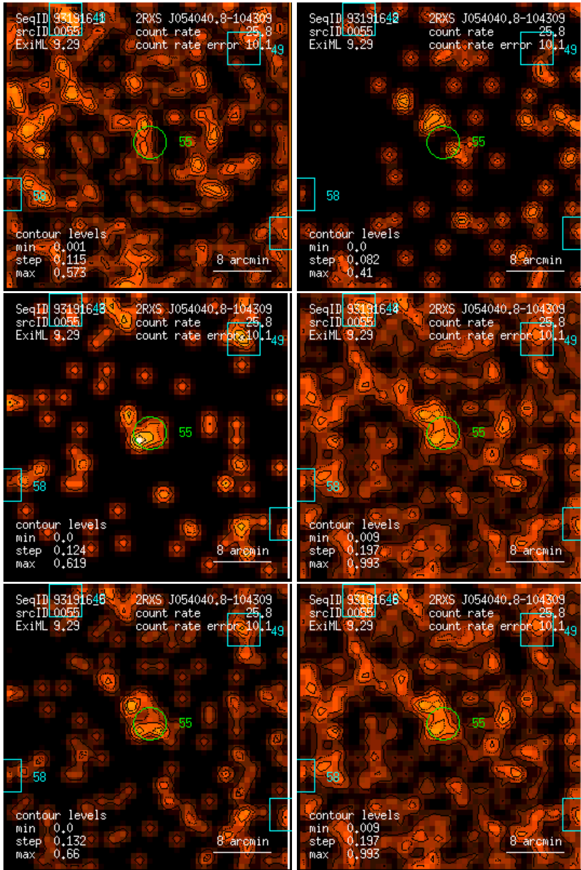
Figure 55: RASS 931916: detection 0055: band rate images, Gaussian filter: (1) PSPC channels 11 – 41, (2) 52 – 90, (3) 91 – 201, (4) 11 – 235, (5) 52 – 201, (6) 11 – 201. Broad band rates in counts/ks. Band rate contour levels in counts/ks/arcmin 2 .
