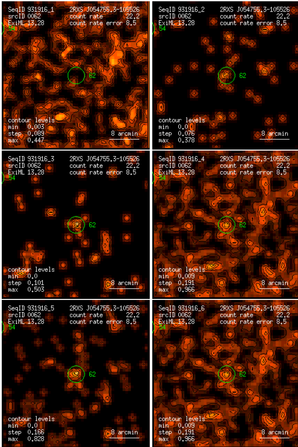
Figure 62: RASS 931916: detection 0062: band rate images, Gaussian filter: (1) PSPC channels 11 – 41, (2) 52 – 90, (3) 91 – 201, (4) 11 – 235, (5) 52 – 201, (6) 11 – 201. Broad band rates in counts/ks. Band rate contour levels in counts/ks/arcmin 2 .
