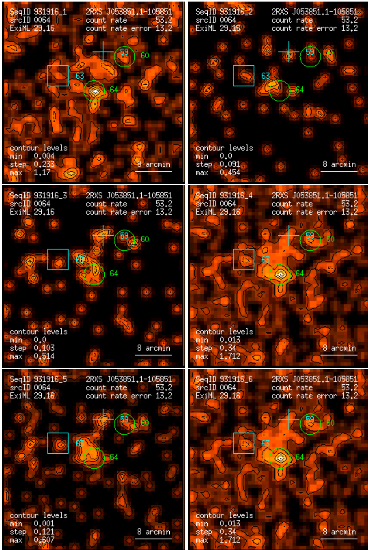
Figure 64: RASS 931916: detection 0064: band rate images, Gaussian filter: (1) PSPC channels 11 – 41, (2) 52 – 90, (3) 91 – 201, (4) 11 – 235, (5) 52 – 201, (6) 11 – 201. Broad band rates in counts/ks. Band rate contour levels in counts/ks/arcmin 2 .
