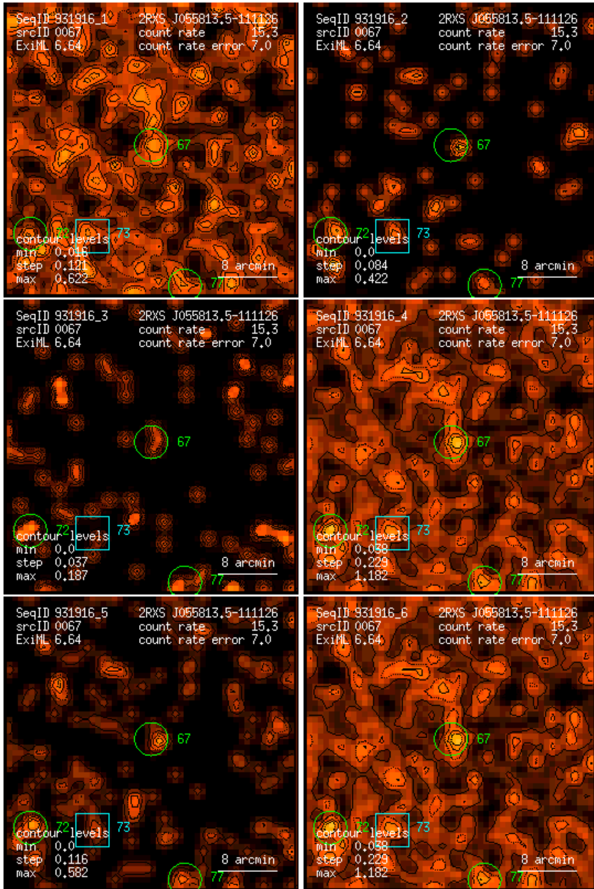
Figure 67: RASS 931916: detection 0067: band rate images, Gaussian filter: (1) PSPC channels 11 – 41, (2) 52 – 90, (3) 91 – 201, (4) 11 – 235, (5) 52 – 201, (6) 11 – 201. Broad band rates in counts/ks. Band rate contour levels in counts/ks/arcmin 2 .
