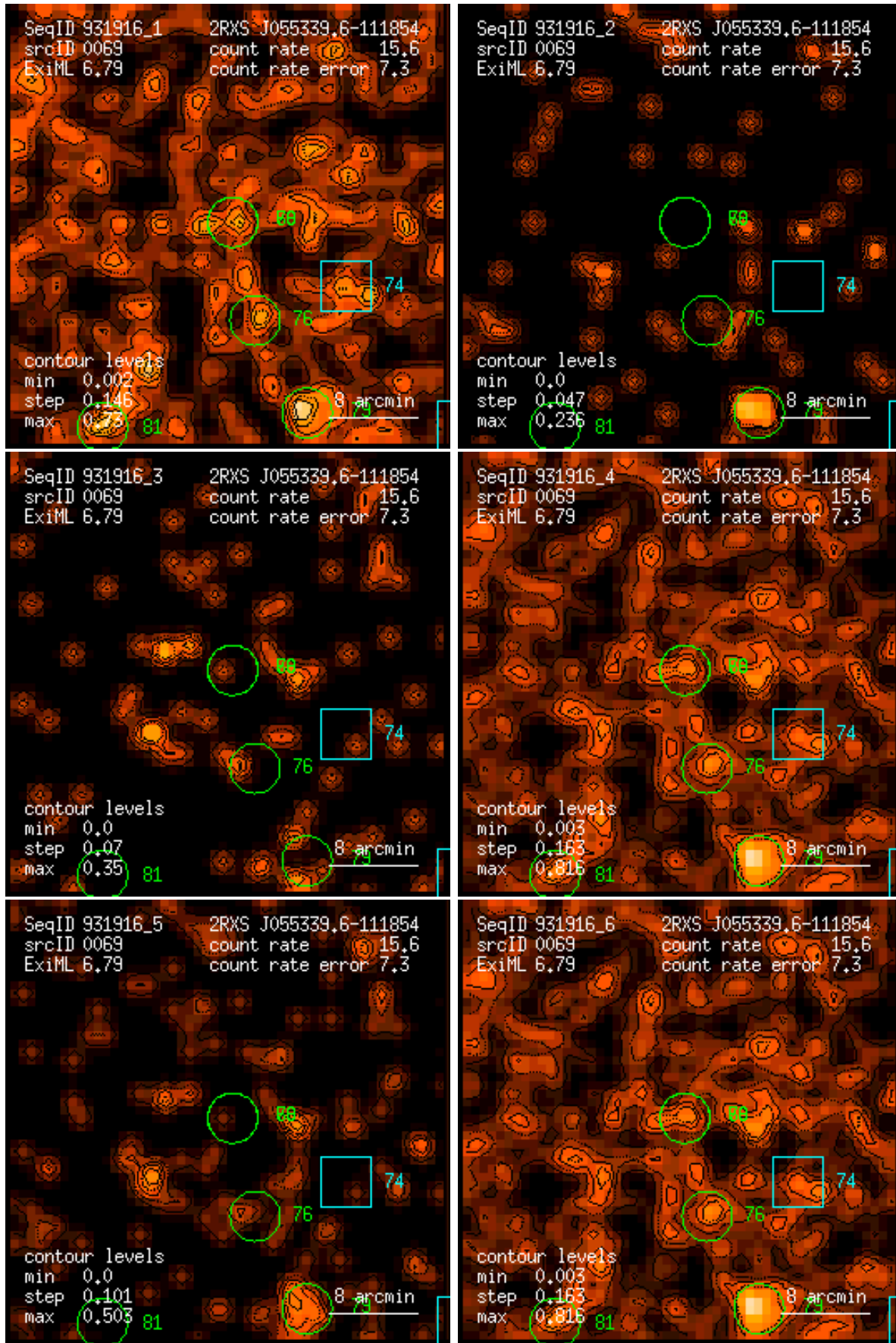
Figure 69: RASS 931916: detection 0069: band rate images, Gaussian filter: (1) PSPC channels 11 – 41, (2) 52 – 90, (3) 91 – 201, (4) 11 – 235, (5) 52 – 201, (6) 11 – 201. Broad band rates in counts/ks. Band rate contour levels in counts/ks/arcmin 2 .
