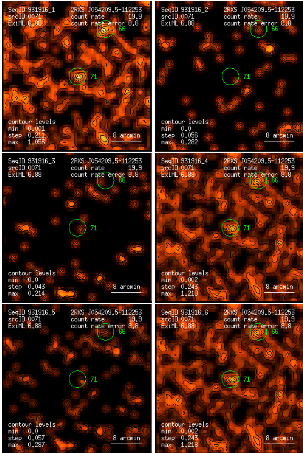
Figure 71: RASS 931916: detection 0071: band rate images, Gaussian filter: (1) PSPC channels 11 – 41, (2) 52 – 90, (3) 91 – 201, (4) 11 – 235, (5) 52 – 201, (6) 11 – 201. Broad band rates in counts/ks. Band rate contour levels in counts/ks/arcmin 2 .
