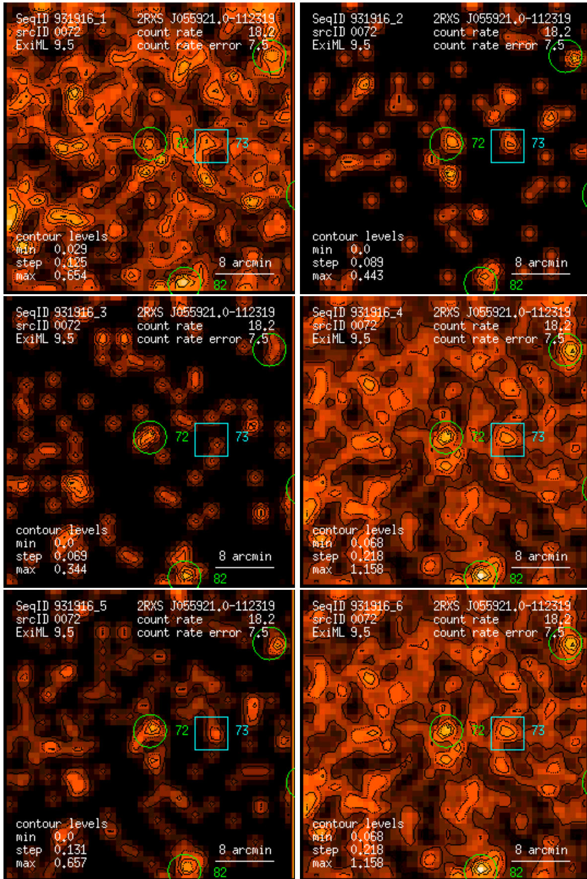
Figure 72: RASS 931916: detection 0072: band rate images, Gaussian filter: (1) PSPC channels 11 – 41, (2) 52 – 90, (3) 91 – 201, (4) 11 – 235, (5) 52 – 201, (6) 11 – 201. Broad band rates in counts/ks. Band rate contour levels in counts/ks/arcmin 2 .
