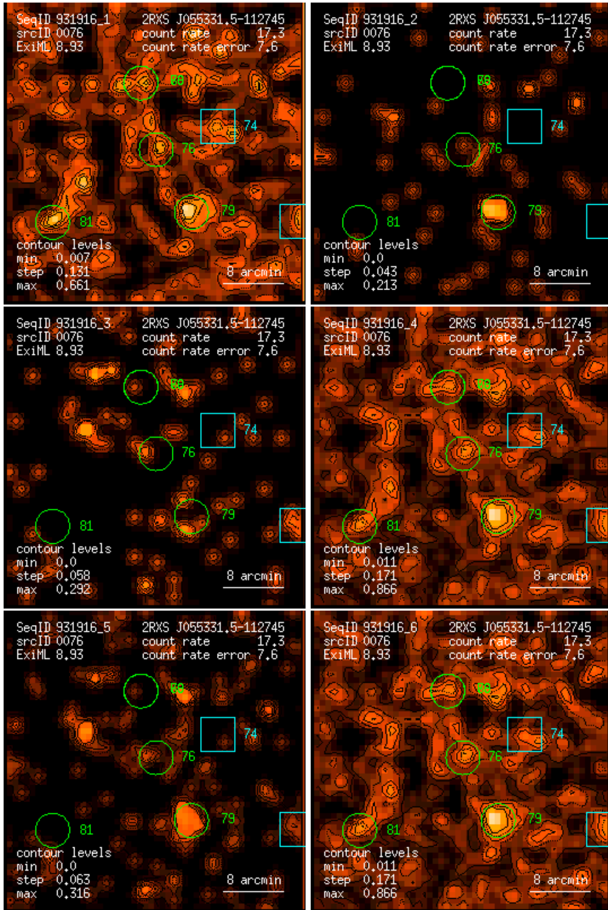
Figure 76: RASS 931916: detection 0076: band rate images, Gaussian filter: (1) PSPC channels 11 – 41, (2) 52 – 90, (3) 91 – 201, (4) 11 – 235, (5) 52 – 201, (6) 11 – 201. Broad band rates in counts/ks. Band rate contour levels in counts/ks/arcmin 2 .
