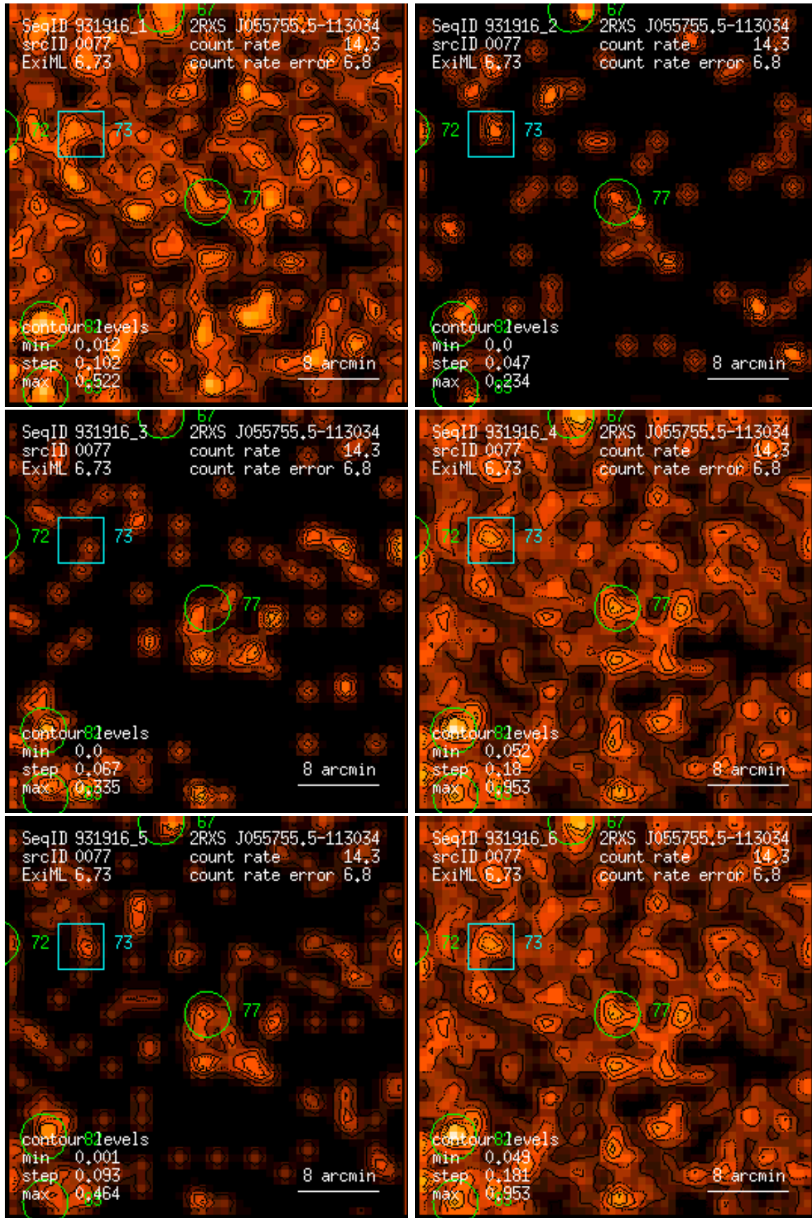
Figure 77: RASS 931916: detection 0077: band rate images, Gaussian filter: (1) PSPC channels 11 – 41, (2) 52 – 90, (3) 91 – 201, (4) 11 – 235, (5) 52 – 201, (6) 11 – 201. Broad band rates in counts/ks. Band rate contour levels in counts/ks/arcmin 2 .
