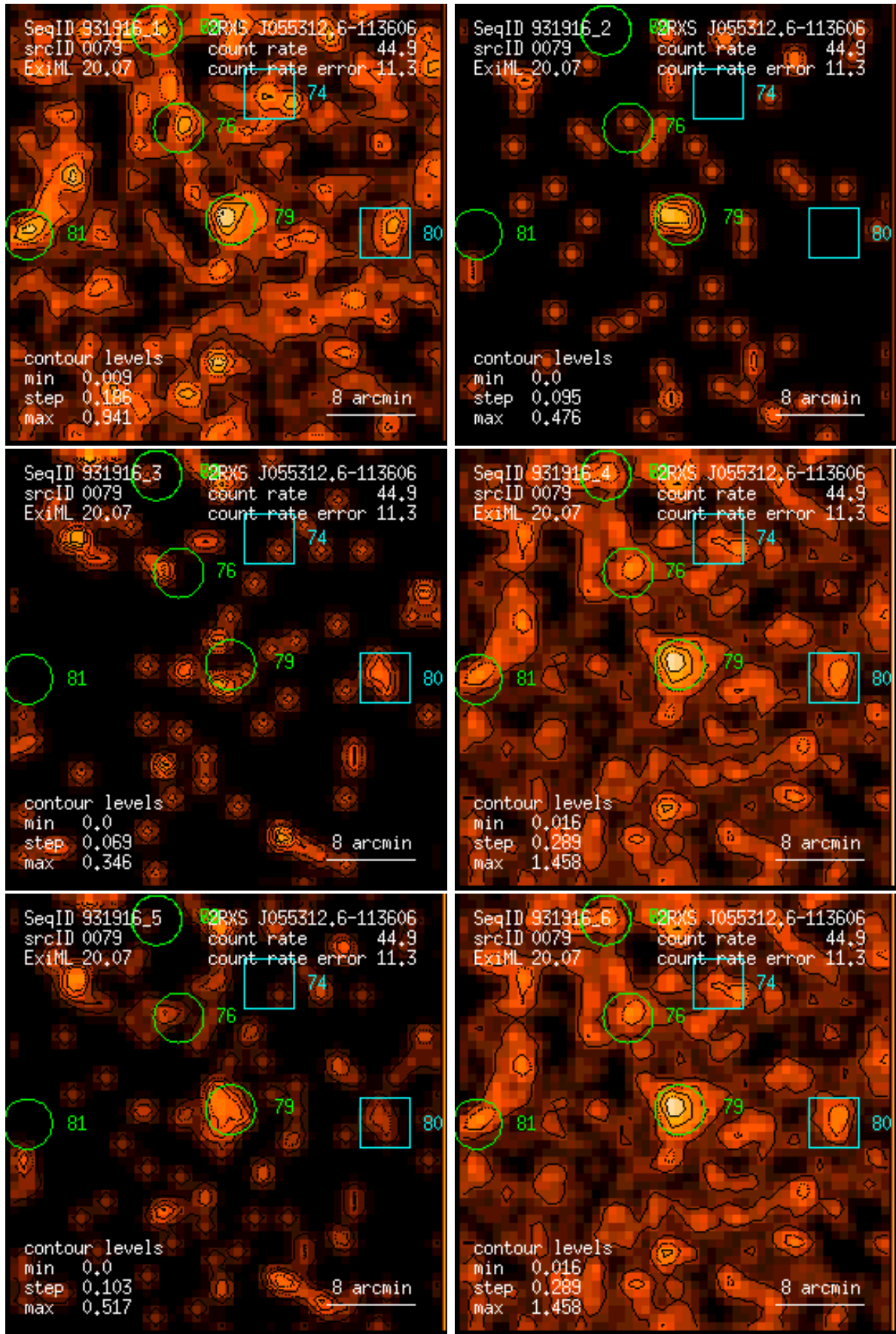
Figure 79: RASS 931916: detection 0079: band rate images, Gaussian filter: (1) PSPC channels 11 – 41, (2) 52 – 90, (3) 91 – 201, (4) 11 – 235, (5) 52 – 201, (6) 11 – 201. Broad band rates in counts/ks. Band rate contour levels in counts/ks/arcmin 2 .
