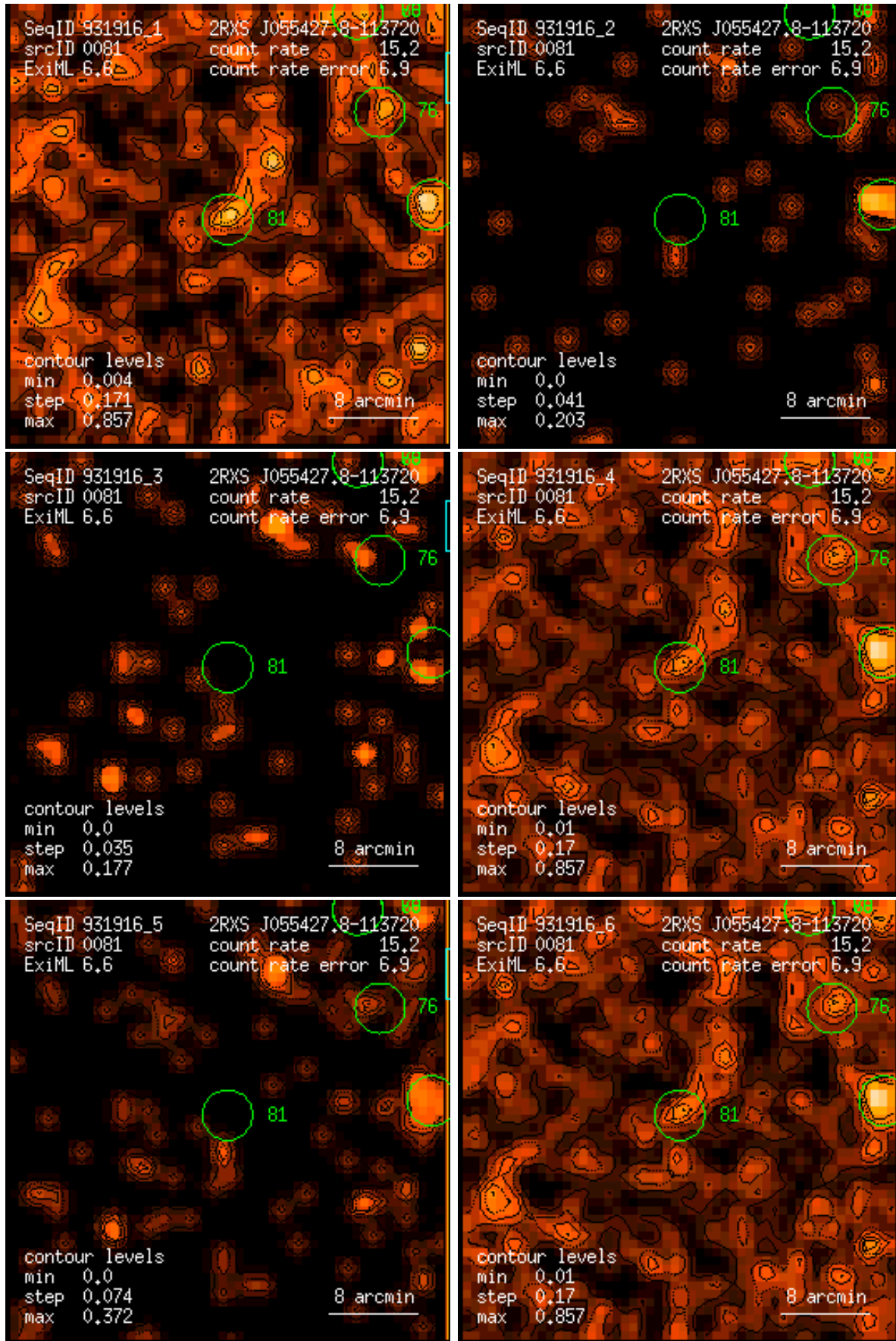
Figure 81: RASS 931916: detection 0081: band rate images, Gaussian filter: (1) PSPC channels 11 – 41, (2) 52 – 90, (3) 91 – 201, (4) 11 – 235, (5) 52 – 201, (6) 11 – 201. Broad band rates in counts/ks. Band rate contour levels in counts/ks/arcmin 2 .
