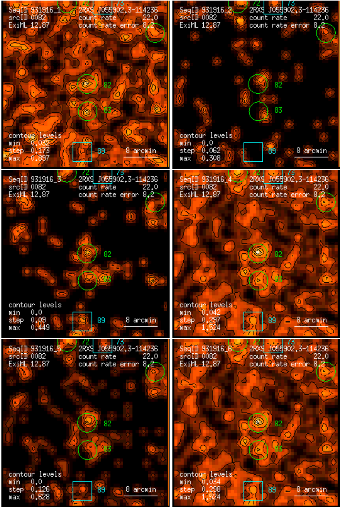
Figure 82: RASS 931916: detection 0082: band rate images, Gaussian filter: (1) PSPC channels 11 – 41, (2) 52 – 90, (3) 91 – 201, (4) 11 – 235, (5) 52 – 201, (6) 11 – 201. Broad band rates in counts/ks. Band rate contour levels in counts/ks/arcmin 2 .
