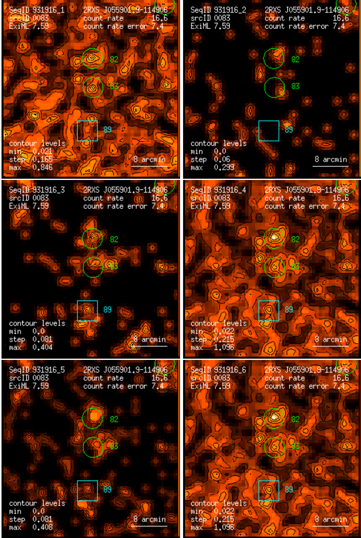
Figure 83: RASS 931916: detection 0083: band rate images, Gaussian filter: (1) PSPC channels 11 – 41, (2) 52 – 90, (3) 91 – 201, (4) 11 – 235, (5) 52 – 201, (6) 11 – 201. Broad band rates in counts/ks. Band rate contour levels in counts/ks/arcmin 2 .
