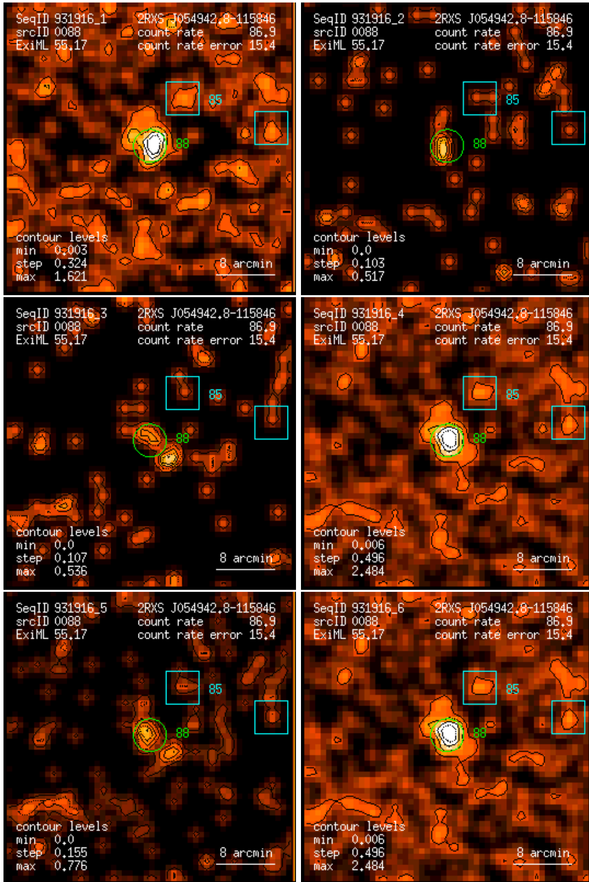
Figure 88: RASS 931916: detection 0088: band rate images, Gaussian filter: (1) PSPC channels 11 – 41, (2) 52 – 90, (3) 91 – 201, (4) 11 – 235, (5) 52 – 201, (6) 11 – 201. Broad band rates in counts/ks. Band rate contour levels in counts/ks/arcmin 2 .
