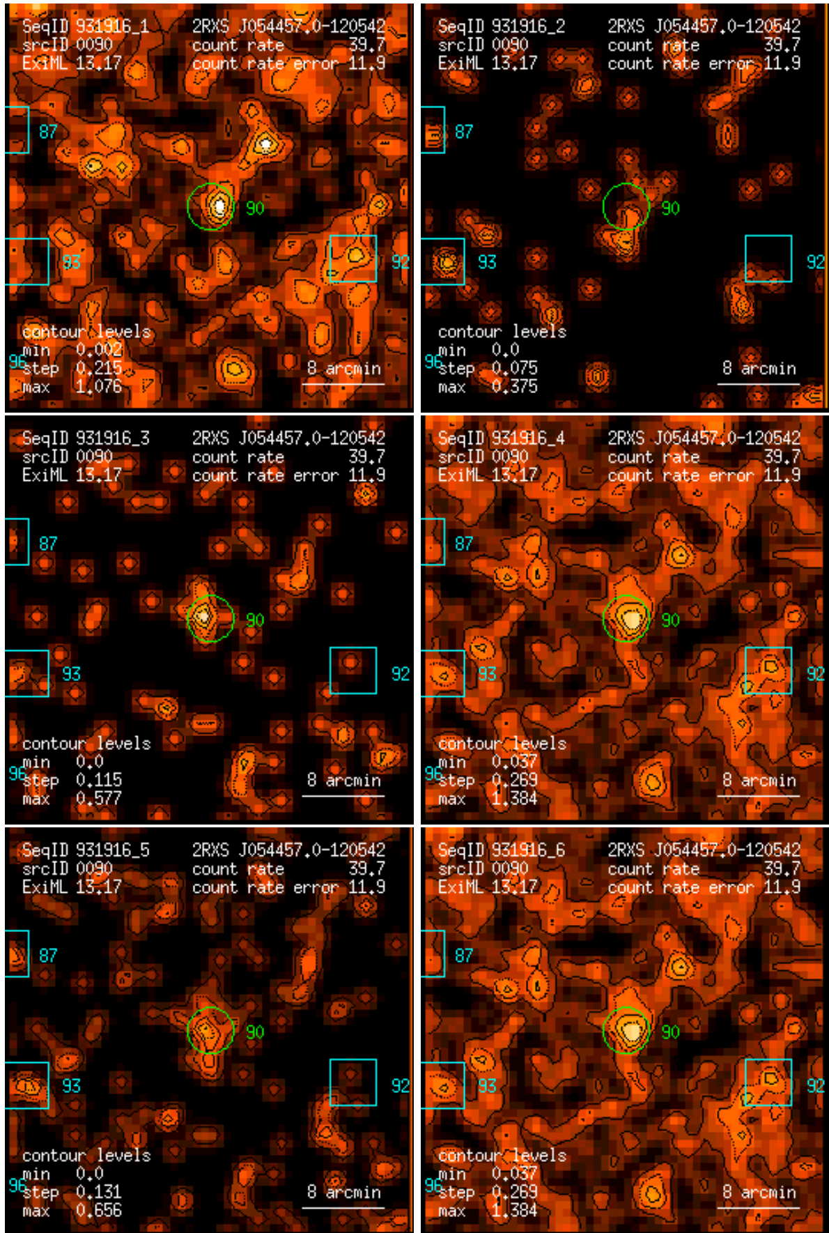
Figure 90: RASS 931916: detection 0090: band rate images, Gaussian filter: (1) PSPC channels 11 – 41, (2) 52 – 90, (3) 91 – 201, (4) 11 – 235, (5) 52 – 201, (6) 11 – 201. Broad band rates in counts/ks. Band rate contour levels in counts/ks/arcmin 2 .
