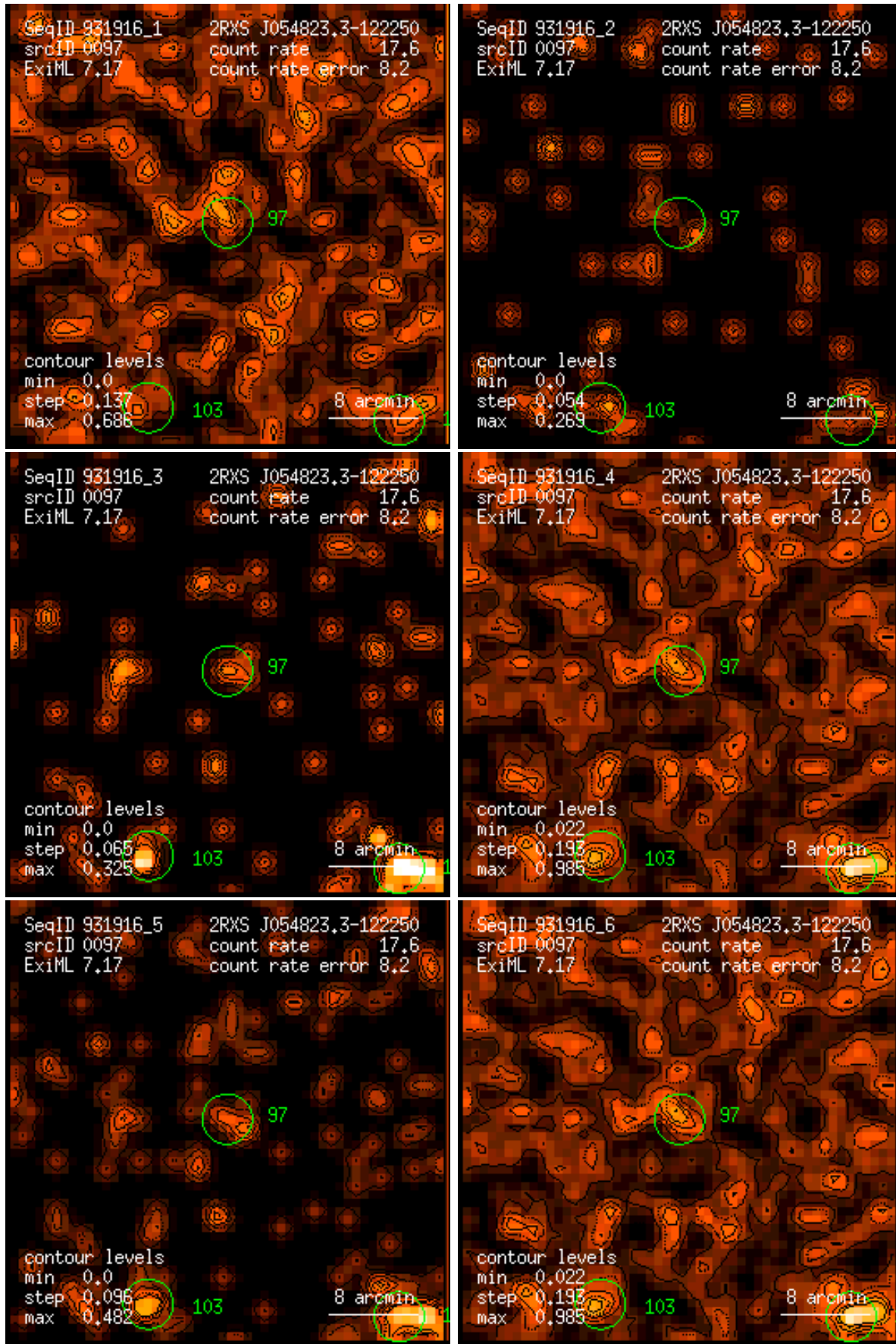
Figure 97: RASS 931916: detection 0097: band rate images, Gaussian filter: (1) PSPC channels 11 – 41, (2) 52 – 90, (3) 91 – 201, (4) 11 – 235, (5) 52 – 201, (6) 11 – 201. Broad band rates in counts/ks. Band rate contour levels in counts/ks/arcmin 2 .
