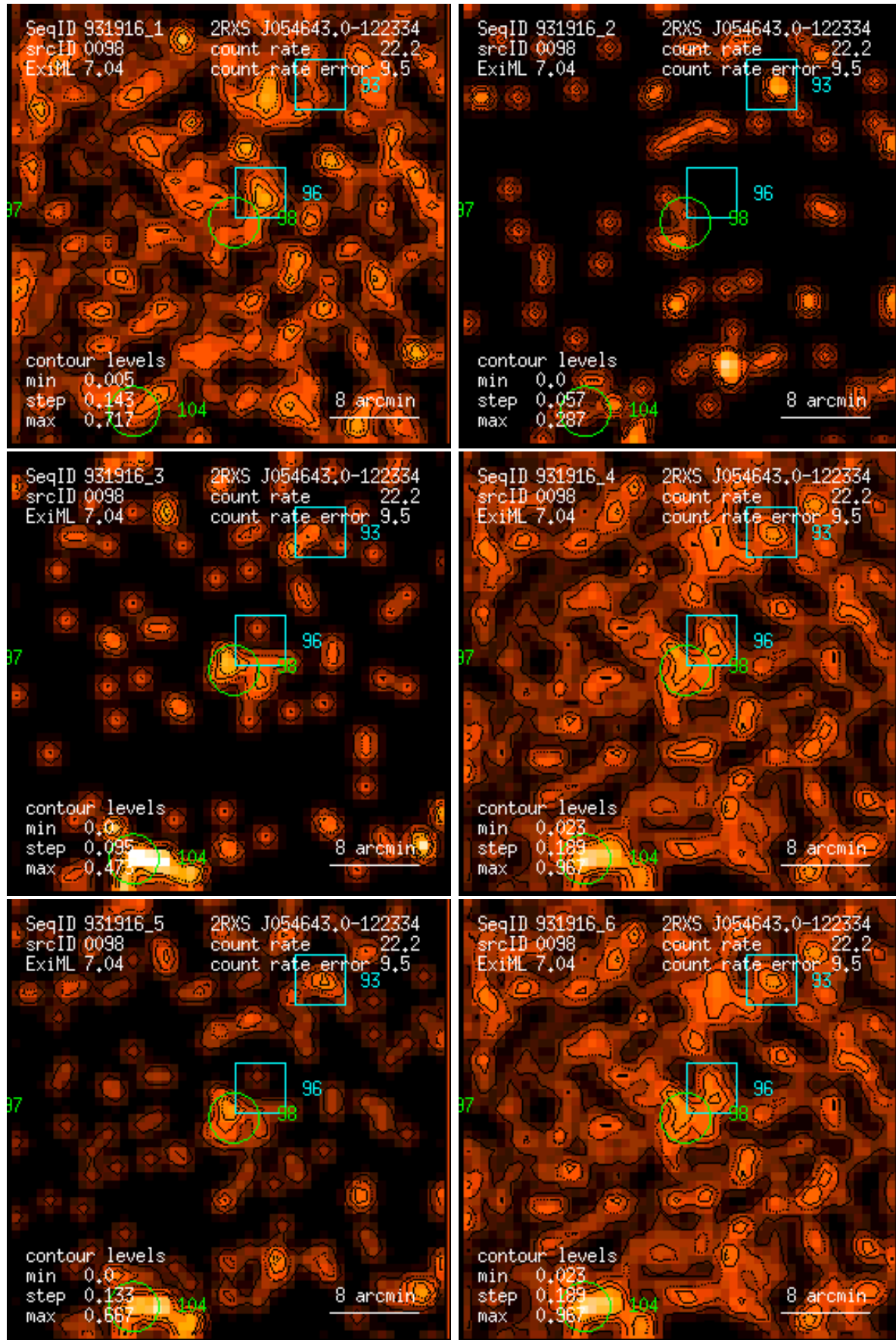
Figure 98: RASS 931916: detection 0098: band rate images, Gaussian filter: (1) PSPC channels 11 – 41, (2) 52 – 90, (3) 91 – 201, (4) 11 – 235, (5) 52 – 201, (6) 11 – 201. Broad band rates in counts/ks. Band rate contour levels in counts/ks/arcmin 2 .
