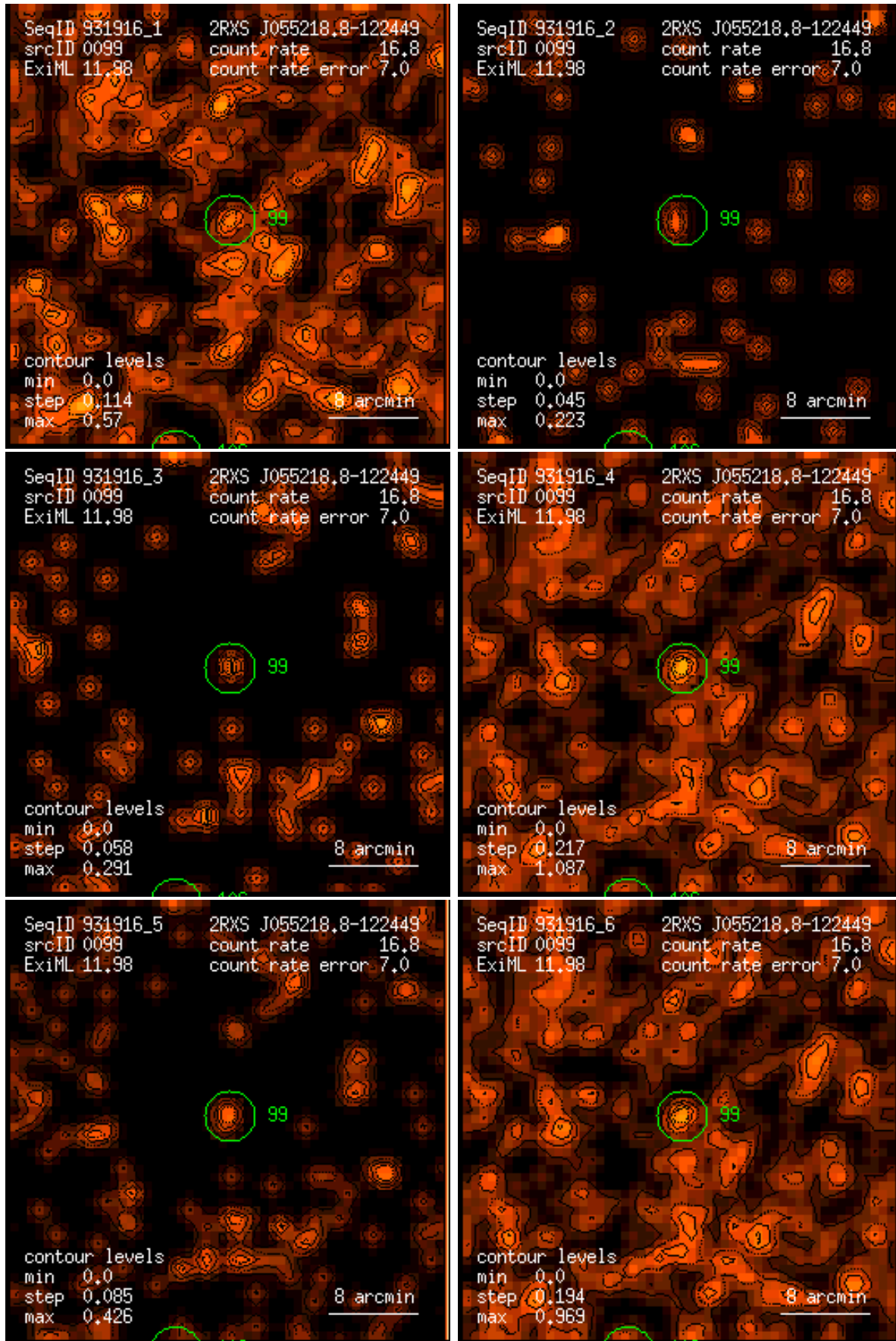
Figure 99: RASS 931916: detection 0099: band rate images, Gaussian filter: (1) PSPC channels 11 – 41, (2) 52 – 90, (3) 91 – 201, (4) 11 – 235, (5) 52 – 201, (6) 11 – 201. Broad band rates in counts/ks. Band rate contour levels in counts/ks/arcmin 2 .
