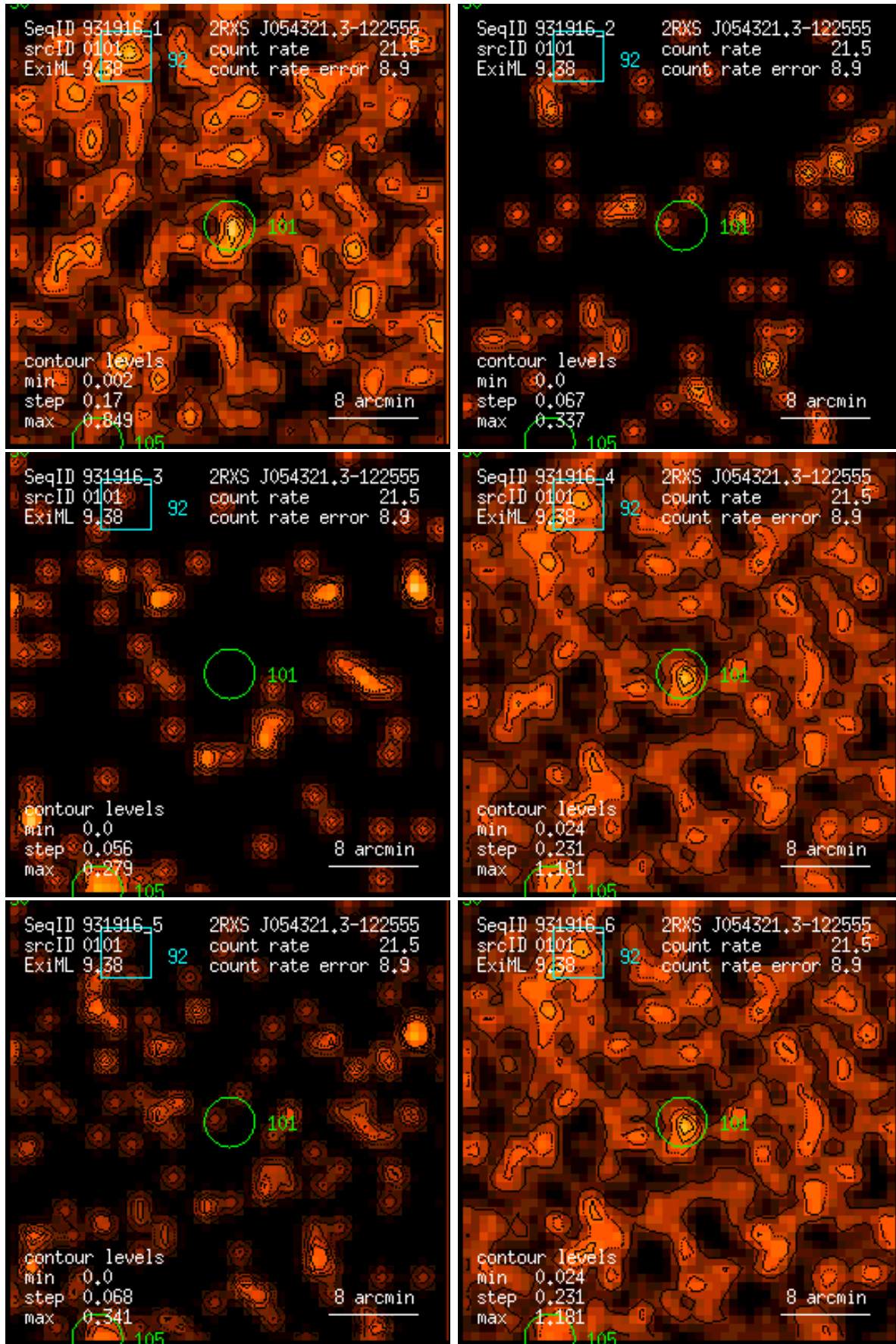
Figure 101: RASS 931916: detection 0101: band rate images, Gaussian filter: (1) PSPC channels 11 – 41, (2) 52 – 90, (3) 91 – 201, (4) 11 – 235, (5) 52 – 201, (6) 11 – 201. Broad band rates in counts/ks. Band rate contour levels in counts/ks/arcmin 2 .
