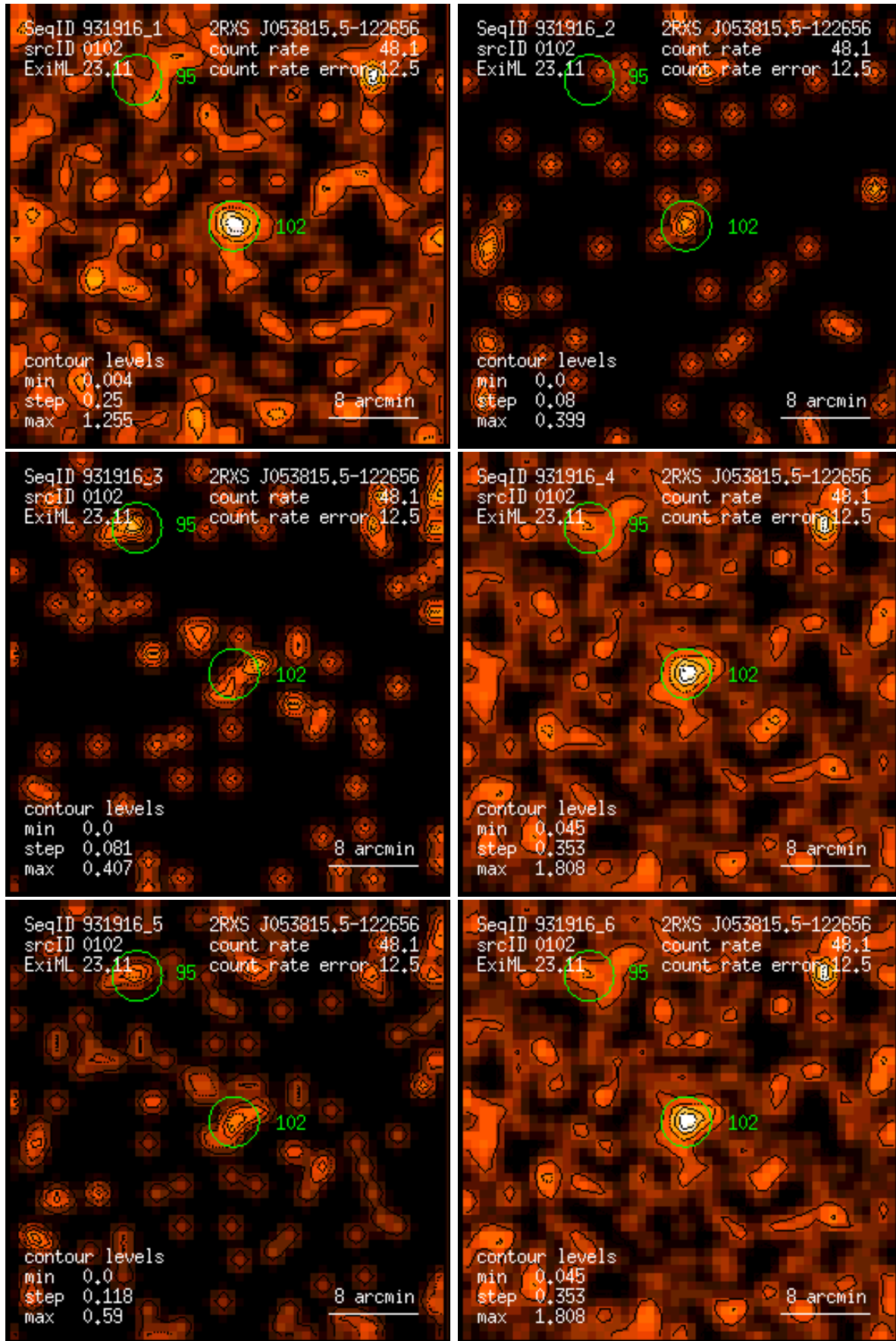
Figure 102: RASS 931916: detection 0102: band rate images, Gaussian filter: (1) PSPC channels 11 – 41, (2) 52 – 90, (3) 91 – 201, (4) 11 – 235, (5) 52 – 201, (6) 11 – 201. Broad band rates in counts/ks. Band rate contour levels in counts/ks/arcmin 2 .
