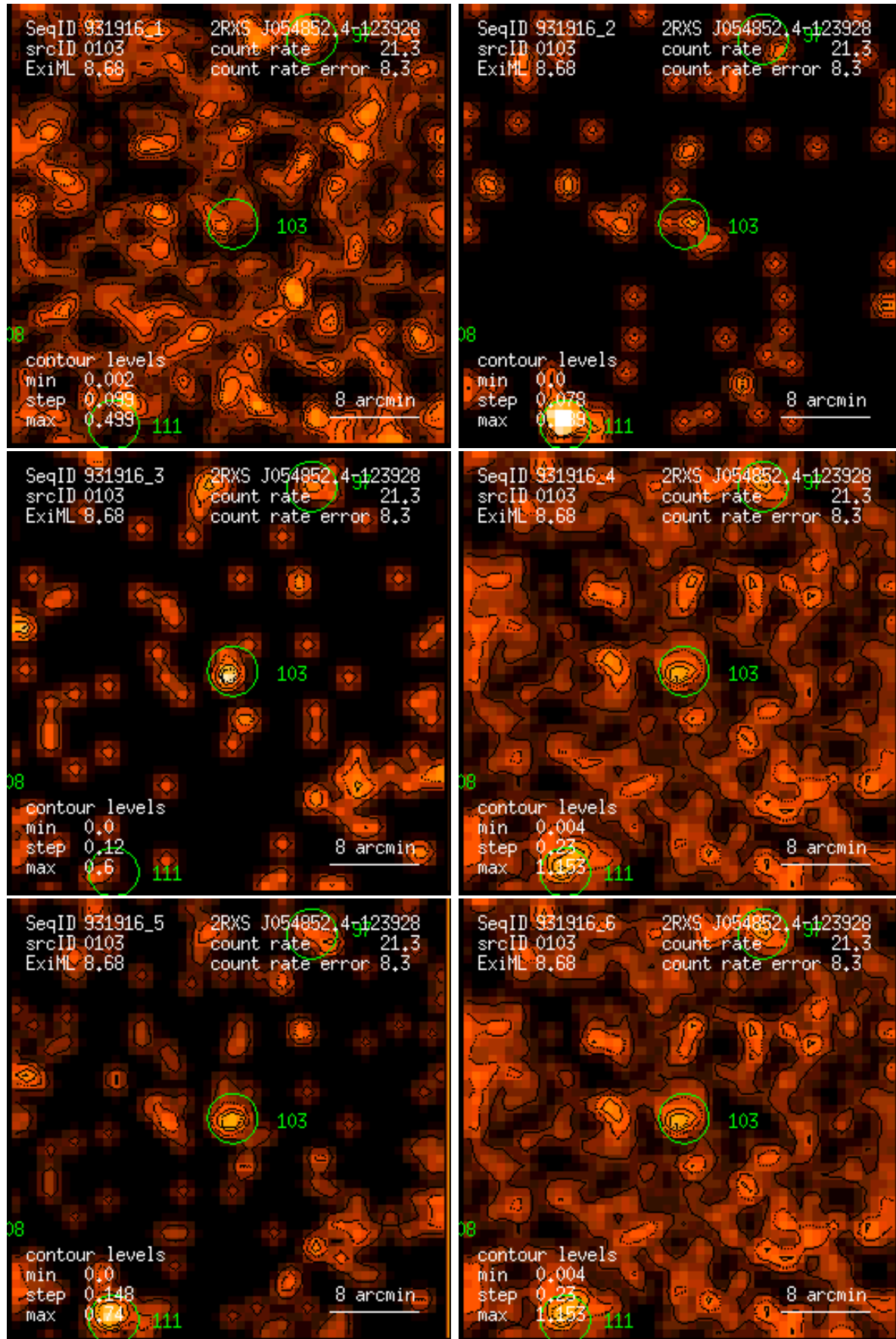
Figure 103: RASS 931916: detection 0103: band rate images, Gaussian filter: (1) PSPC channels 11 – 41, (2) 52 – 90, (3) 91 – 201, (4) 11 – 235, (5) 52 – 201, (6) 11 – 201. Broad band rates in counts/ks. Band rate contour levels in counts/ks/arcmin 2 .
