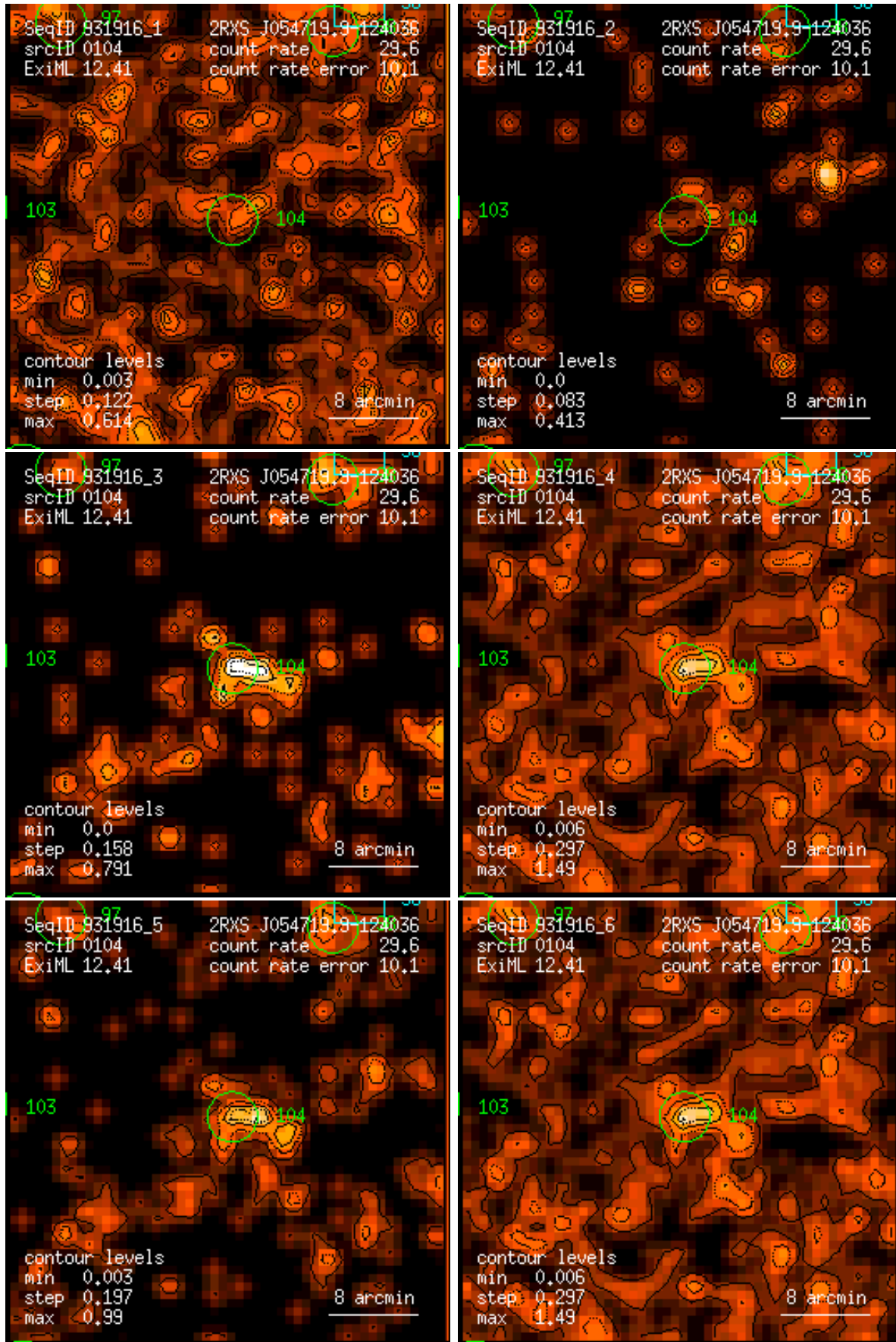
Figure 104: RASS 931916: detection 0104: band rate images, Gaussian filter: (1) PSPC channels 11 – 41, (2) 52 – 90, (3) 91 – 201, (4) 11 – 235, (5) 52 – 201, (6) 11 – 201. Broad band rates in counts/ks. Band rate contour levels in counts/ks/arcmin 2 .
