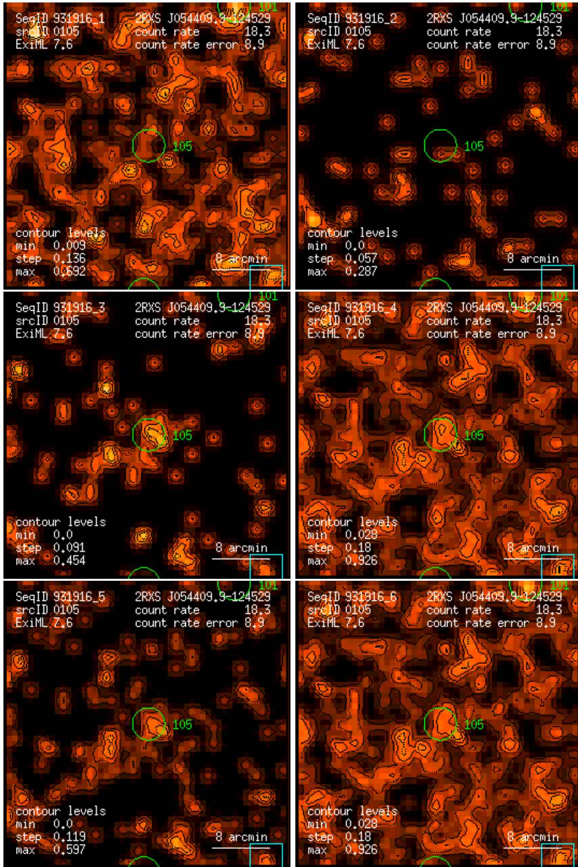
Figure 105: RASS 931916: detection 0105: band rate images, Gaussian filter: (1) PSPC channels 11 – 41, (2) 52 – 90, (3) 91 – 201, (4) 11 – 235, (5) 52 – 201, (6) 11 – 201. Broad band rates in counts/ks. Band rate contour levels in counts/ks/arcmin 2 .
