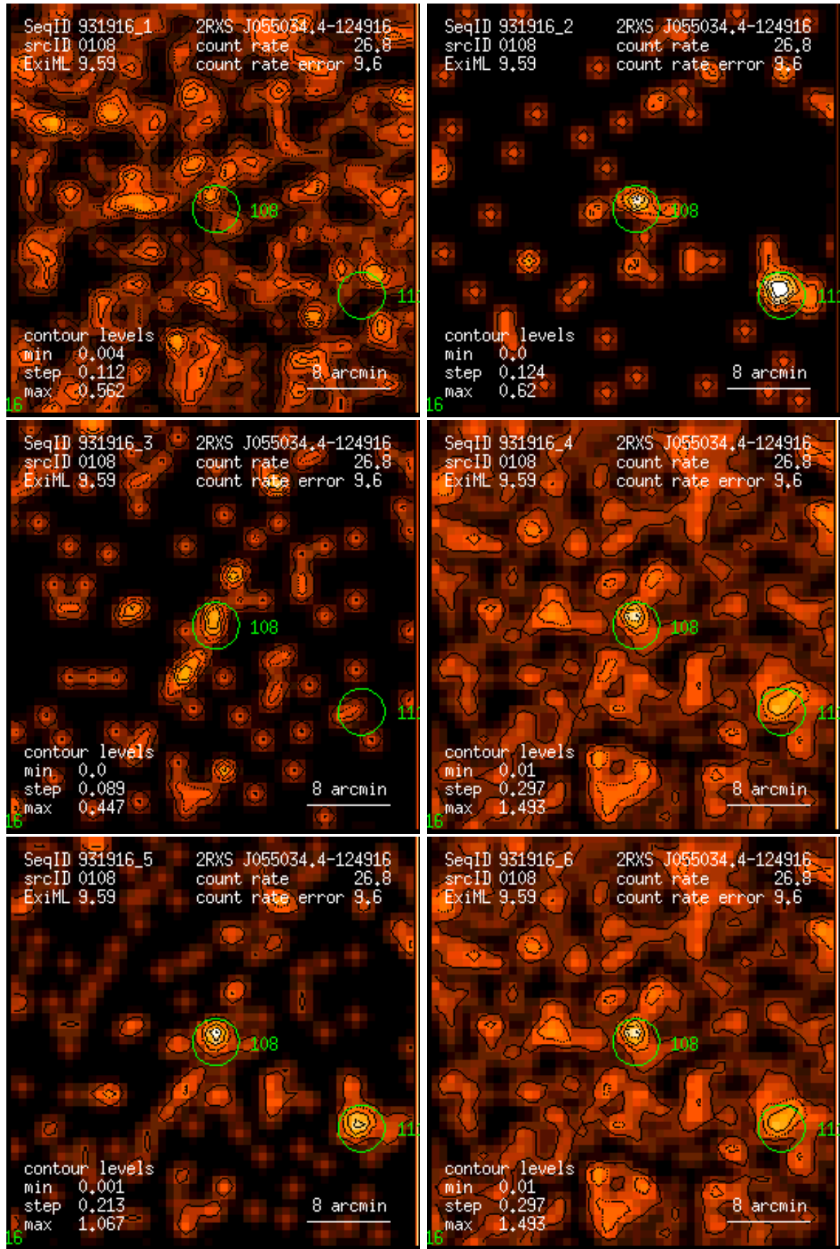
Figure 108: RASS 931916: detection 0108: band rate images, Gaussian filter: (1) PSPC channels 11 – 41, (2) 52 – 90, (3) 91 – 201, (4) 11 – 235, (5) 52 – 201, (6) 11 – 201. Broad band rates in counts/ks. Band rate contour levels in counts/ks/arcmin 2 .
