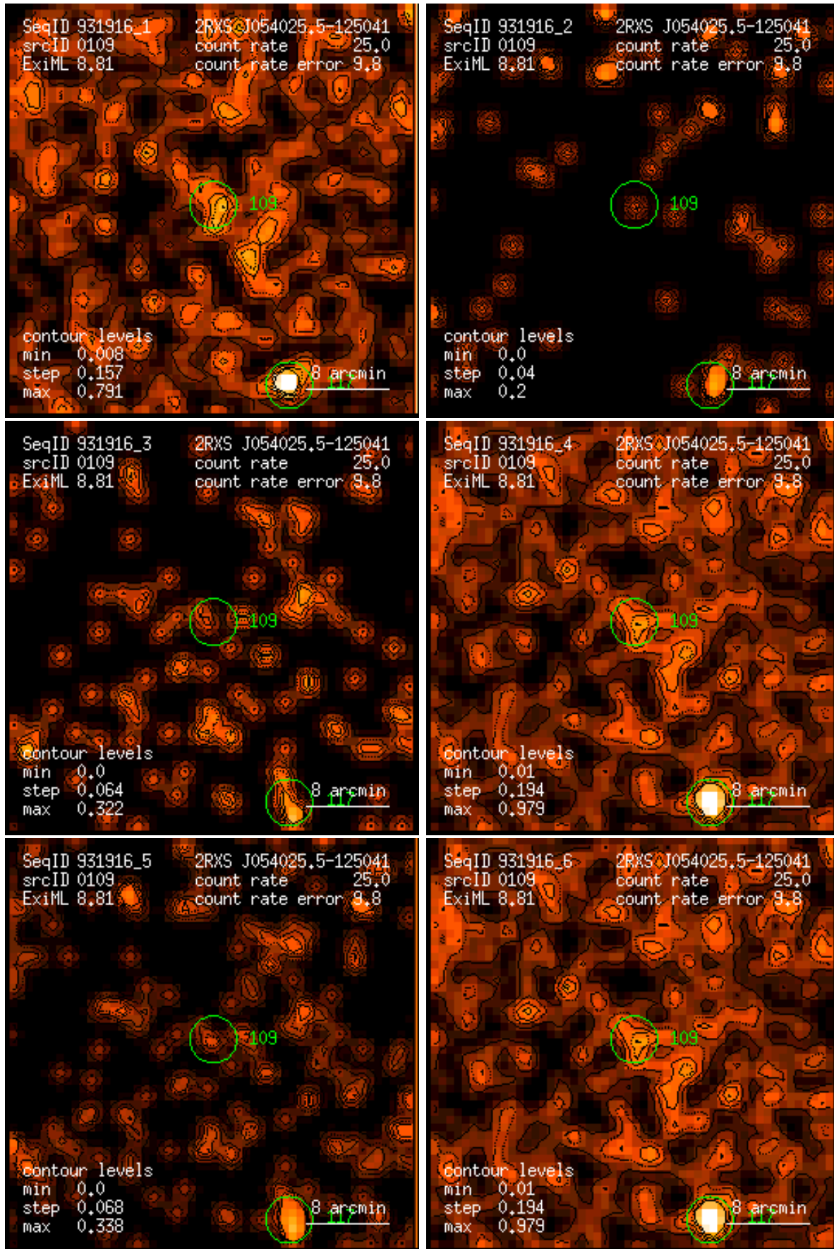
Figure 109: RASS 931916: detection 0109: band rate images, Gaussian filter: (1) PSPC channels 11 – 41, (2) 52 – 90, (3) 91 – 201, (4) 11 – 235, (5) 52 – 201, (6) 11 – 201. Broad band rates in counts/ks. Band rate contour levels in counts/ks/arcmin 2 .
