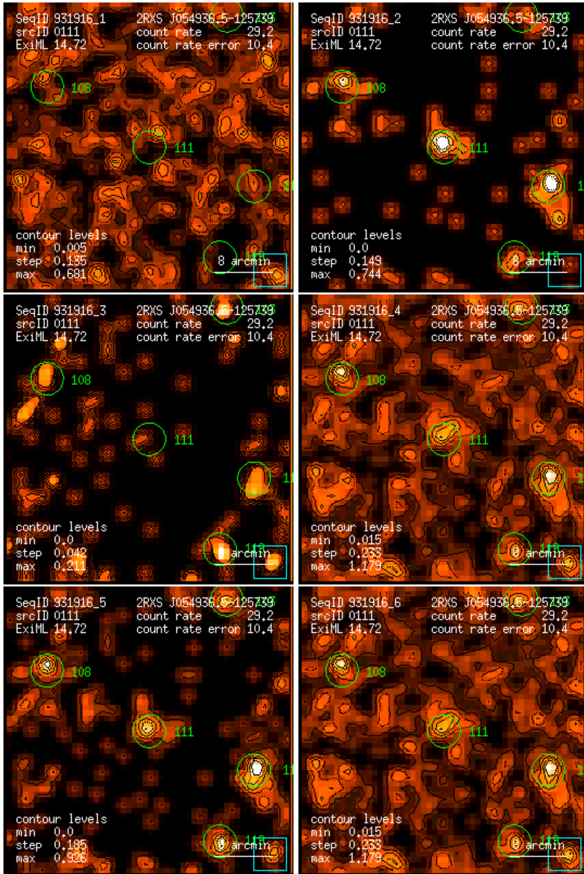
Figure 111: RASS 931916: detection 0111: band rate images, Gaussian filter: (1) PSPC channels 11 – 41, (2) 52 – 90, (3) 91 – 201, (4) 11 – 235, (5) 52 – 201, (6) 11 – 201. Broad band rates in counts/ks. Band rate contour levels in counts/ks/arcmin 2 .
