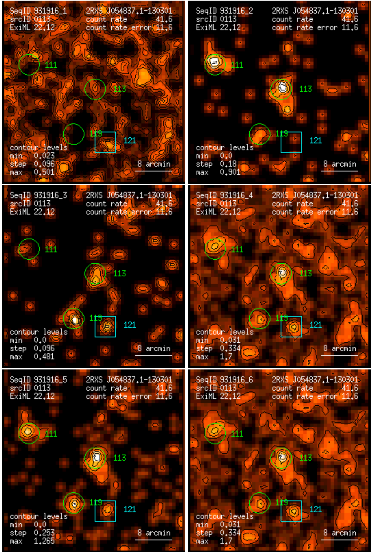
Figure 113: RASS 931916: detection 0113: band rate images, Gaussian filter: (1) PSPC channels 11 – 41, (2) 52 – 90, (3) 91 – 201, (4) 11 – 235, (5) 52 – 201, (6) 11 – 201. Broad band rates in counts/ks. Band rate contour levels in counts/ks/arcmin 2 .
