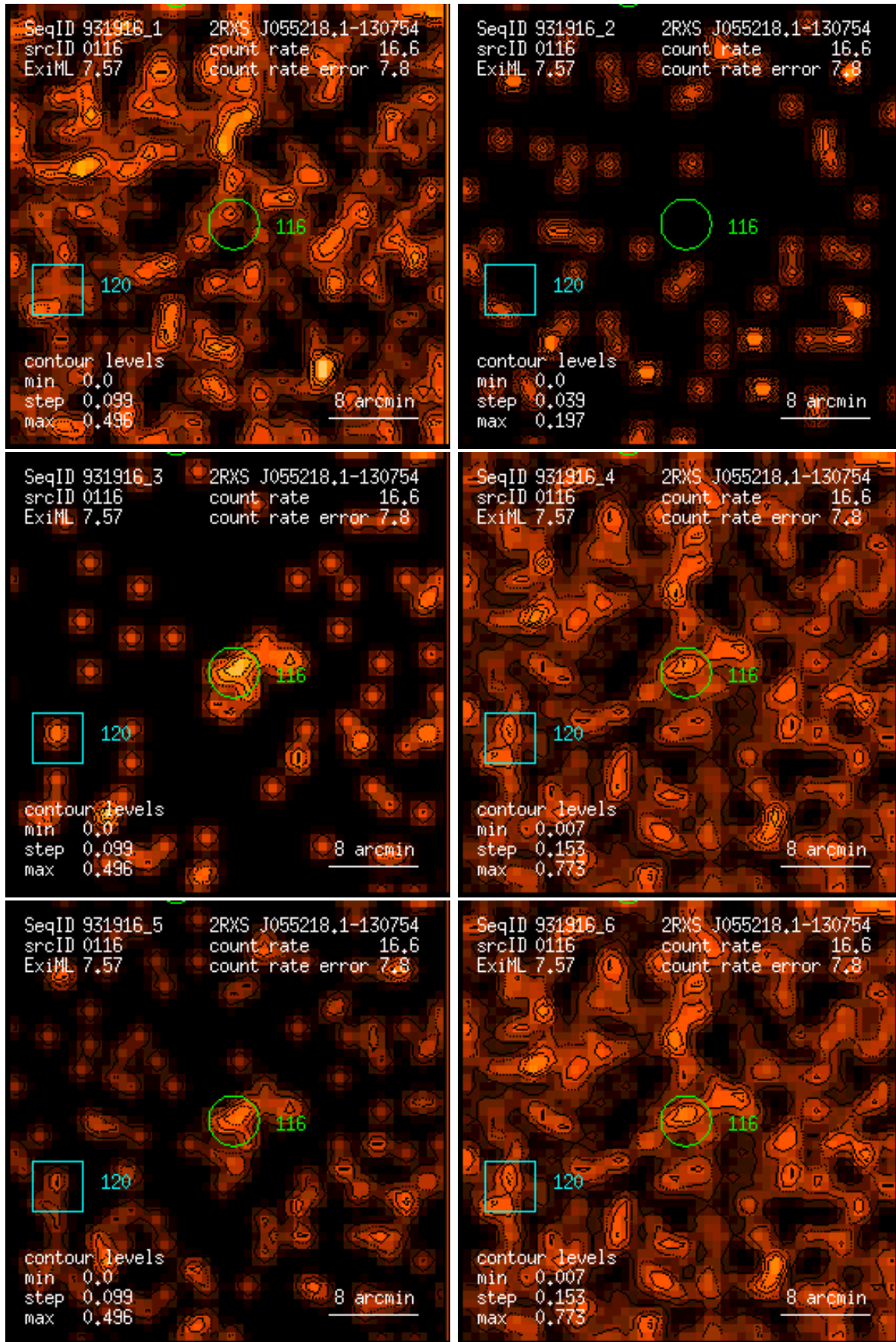
Figure 116: RASS 931916: detection 0116: band rate images, Gaussian filter: (1) PSPC channels 11 – 41, (2) 52 – 90, (3) 91 – 201, (4) 11 – 235, (5) 52 – 201, (6) 11 – 201. Broad band rates in counts/ks. Band rate contour levels in counts/ks/arcmin 2 .
