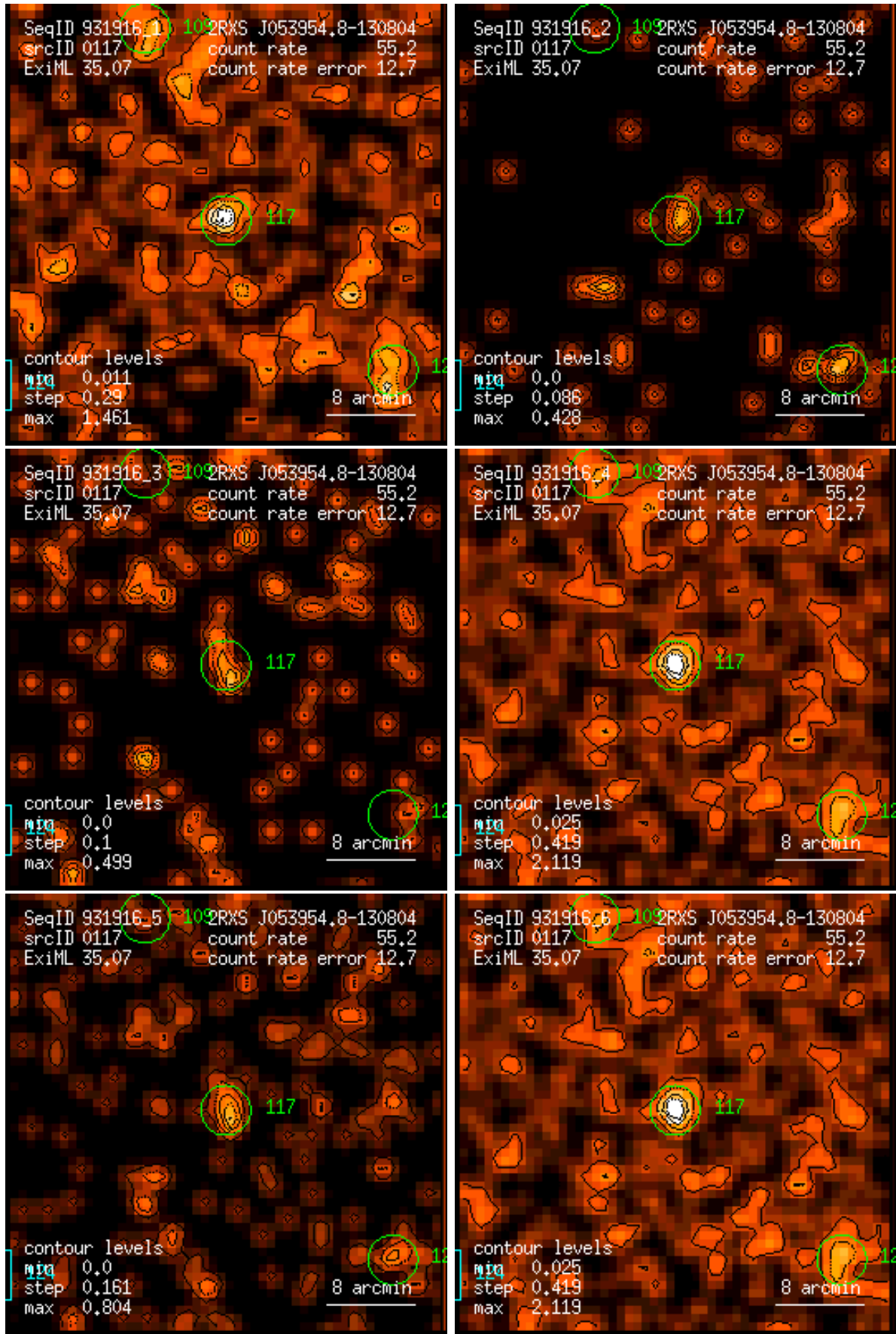
Figure 117: RASS 931916: detection 0117: band rate images, Gaussian filter: (1) PSPC channels 11 – 41, (2) 52 – 90, (3) 91 – 201, (4) 11 – 235, (5) 52 – 201, (6) 11 – 201. Broad band rates in counts/ks. Band rate contour levels in counts/ks/arcmin 2 .
