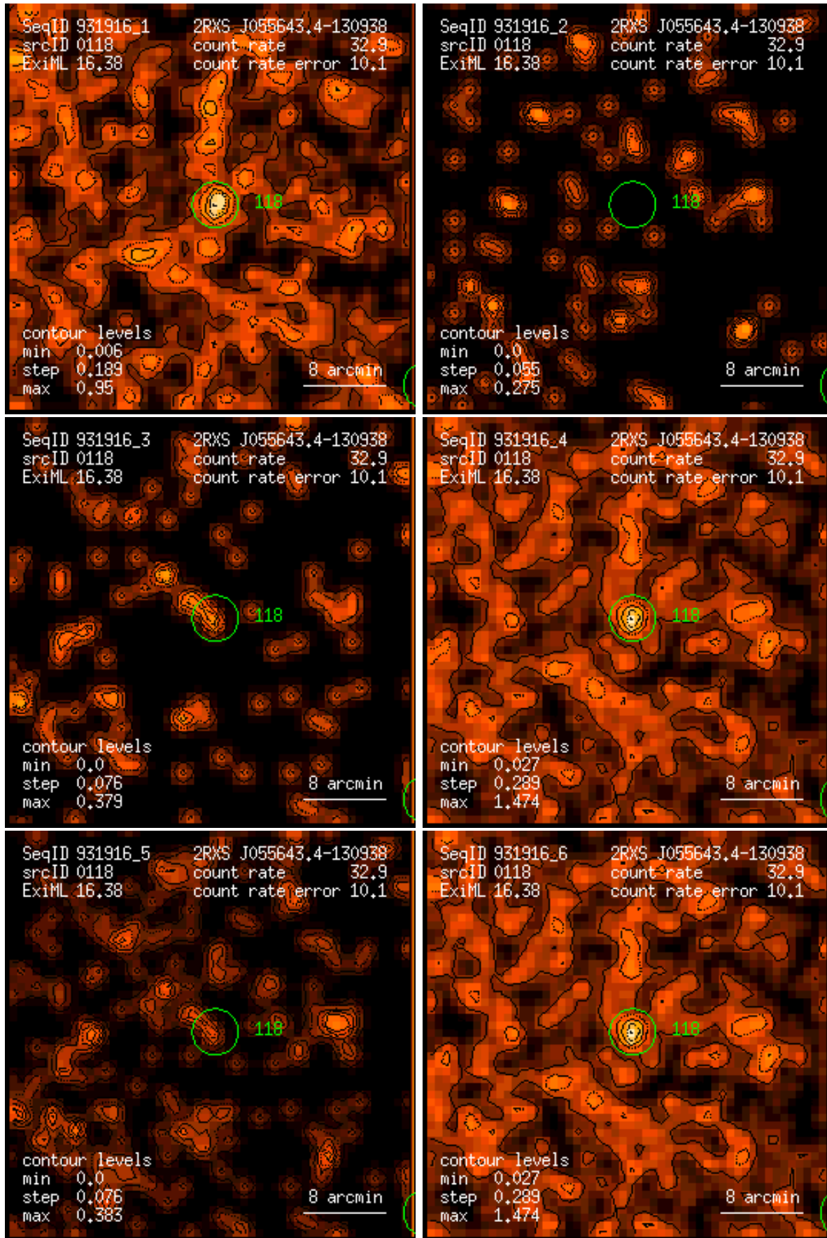
Figure 118: RASS 931916: detection 0118: band rate images, Gaussian filter: (1) PSPC channels 11 – 41, (2) 52 – 90, (3) 91 – 201, (4) 11 – 235, (5) 52 – 201, (6) 11 – 201. Broad band rates in counts/ks. Band rate contour levels in counts/ks/arcmin 2 .
