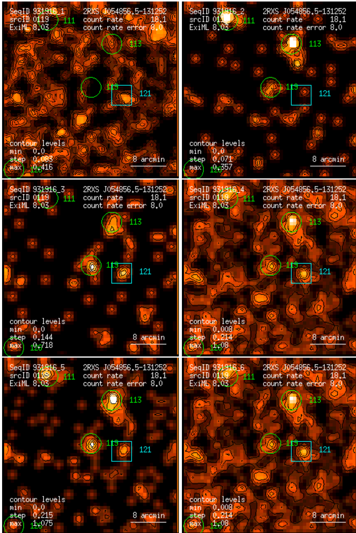
Figure 119: RASS 931916: detection 0119: band rate images, Gaussian filter: (1) PSPC channels 11 – 41, (2) 52 – 90, (3) 91 – 201, (4) 11 – 235, (5) 52 – 201, (6) 11 – 201. Broad band rates in counts/ks. Band rate contour levels in counts/ks/arcmin 2 .
