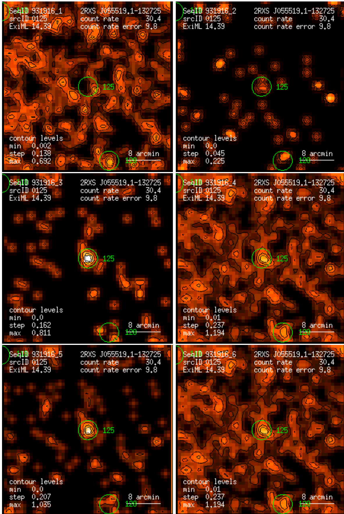
Figure 125: RASS 931916: detection 0125: band rate images, Gaussian filter: (1) PSPC channels 11 – 41, (2) 52 – 90, (3) 91 – 201, (4) 11 – 235, (5) 52 – 201, (6) 11 – 201. Broad band rates in counts/ks. Band rate contour levels in counts/ks/arcmin 2 .
