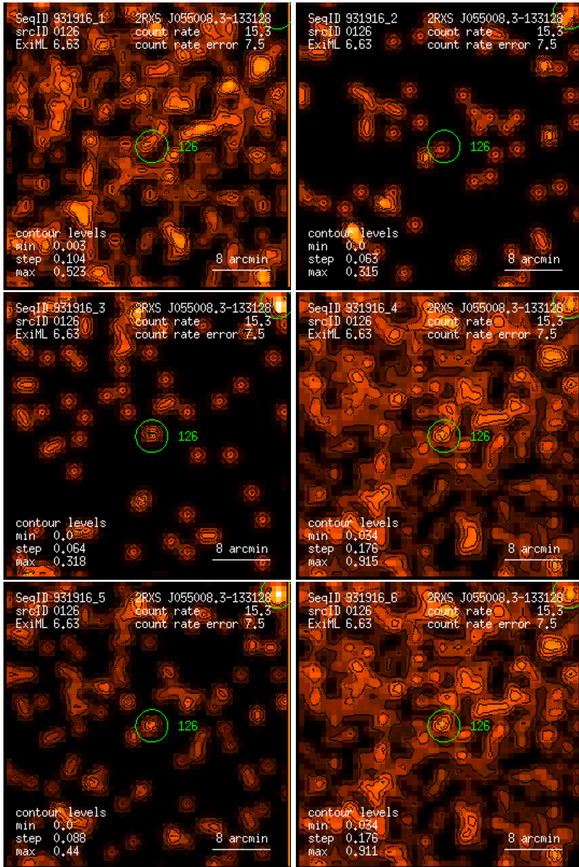
Figure 126: RASS 931916: detection 0126: band rate images, Gaussian filter: (1) PSPC channels 11 – 41, (2) 52 – 90, (3) 91 – 201, (4) 11 – 235, (5) 52 – 201, (6) 11 – 201. Broad band rates in counts/ks. Band rate contour levels in counts/ks/arcmin 2 .
