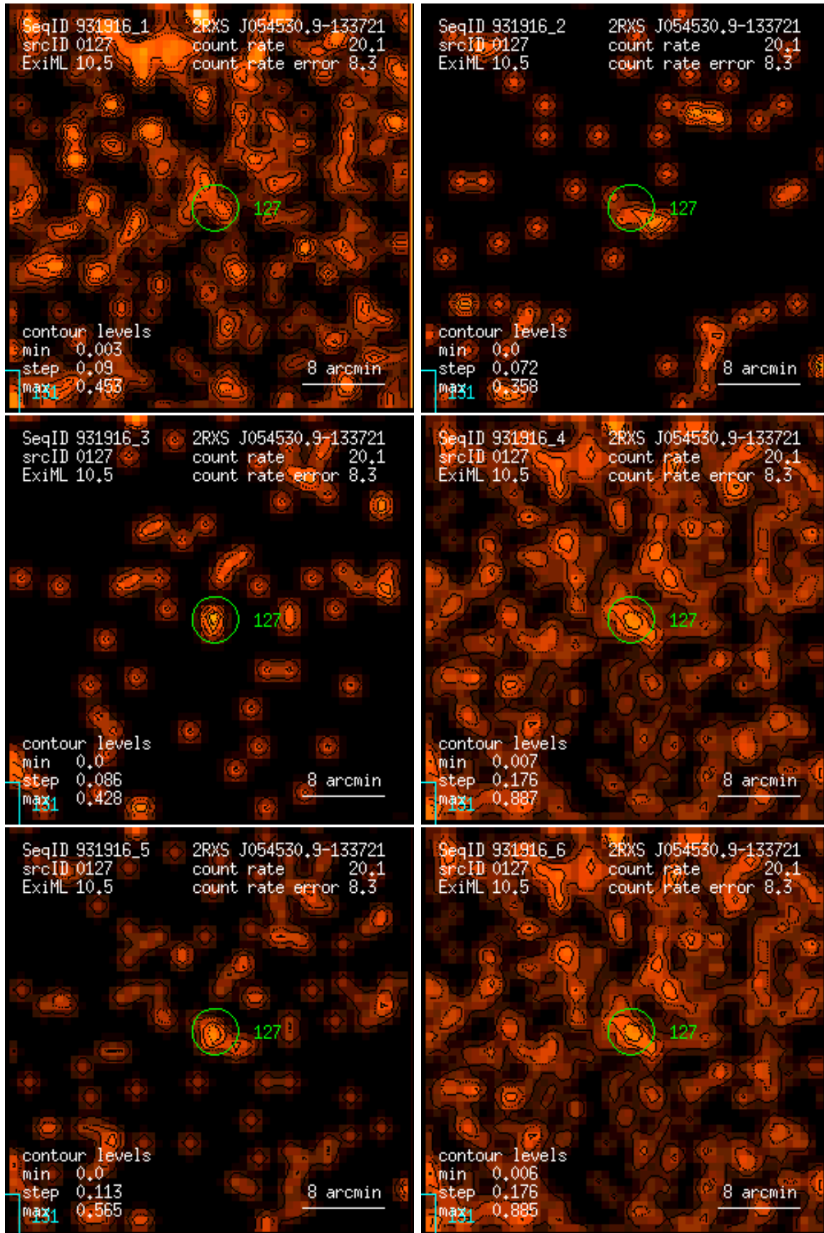
Figure 127: RASS 931916: detection 0127: band rate images, Gaussian filter: (1) PSPC channels 11 – 41, (2) 52 – 90, (3) 91 – 201, (4) 11 – 235, (5) 52 – 201, (6) 11 – 201. Broad band rates in counts/ks. Band rate contour levels in counts/ks/arcmin 2 .
