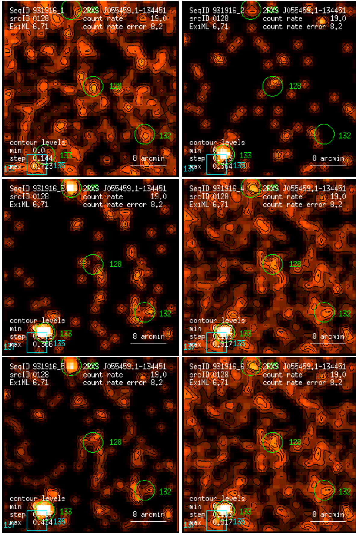
Figure 128: RASS 931916: detection 0128: band rate images, Gaussian filter: (1) PSPC channels 11 – 41, (2) 52 – 90, (3) 91 – 201, (4) 11 – 235, (5) 52 – 201, (6) 11 – 201. Broad band rates in counts/ks. Band rate contour levels in counts/ks/arcmin 2 .
